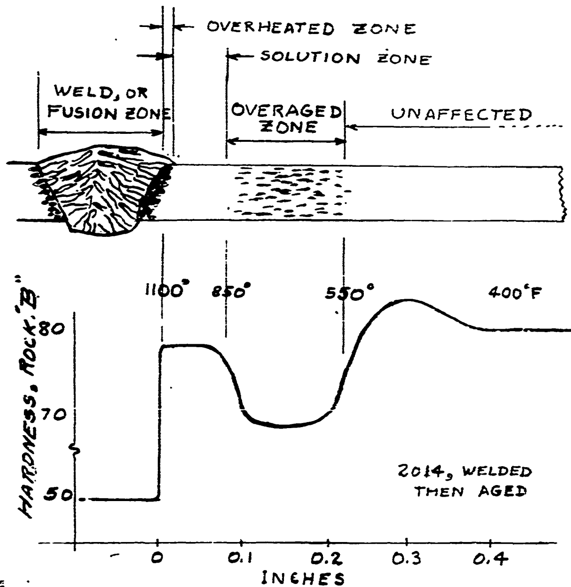
THE HEAT-AFFECTED ZONES WITH APPROX. THERMAL GRADIENT & HARDNESS SURVEY.
