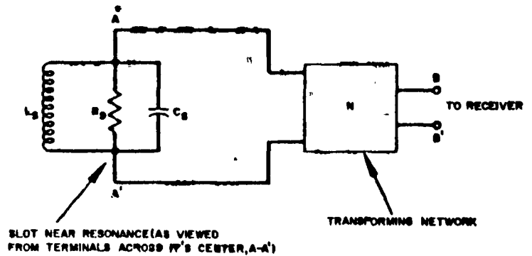
Figure 4. Equivalent circuit of slot near resonance. Network N transforms parallel arrangement at A-A' to series RLC circuit at B-B'. This is then connected in shunt with feed waveguide.
