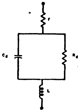
Figure 3. Equivalent circuit of tunnel diode.
