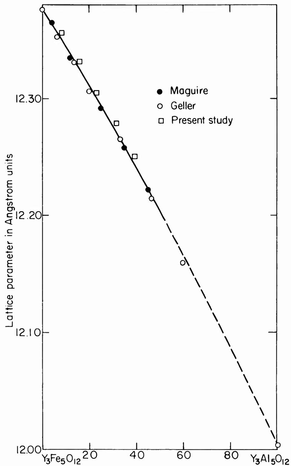
LATTICE PARAMETERS OF Y_3Fe_5O_{12} - Y_3Al_5O_{12} SOLID SOLUTIONS FIGURE 5
