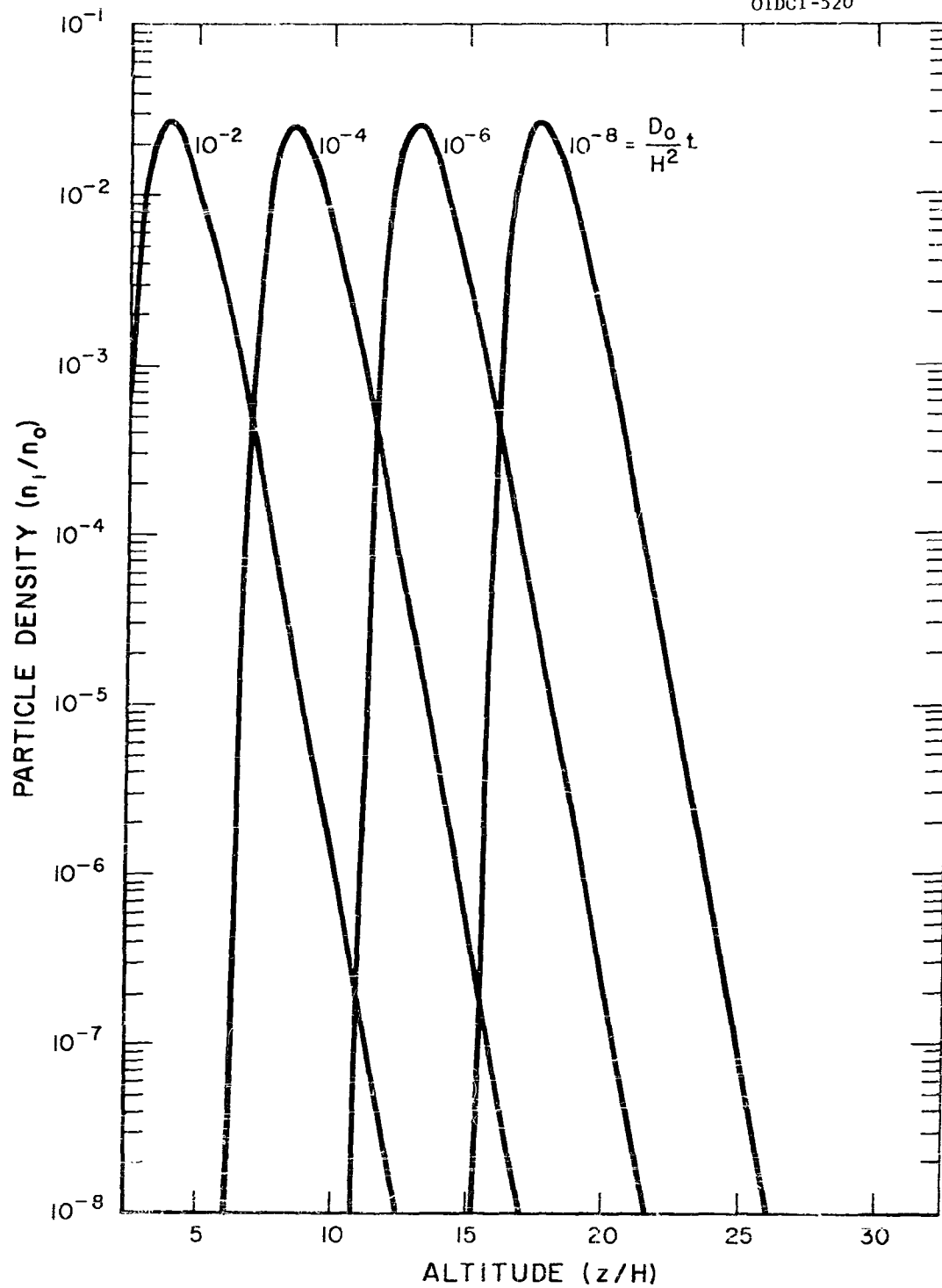
Figure 2. Particle density function \frac{n_1}{n_0} as a function of altitude for several values of time \frac{D_0}{H^2} t ; mass ratio a = 2 .
