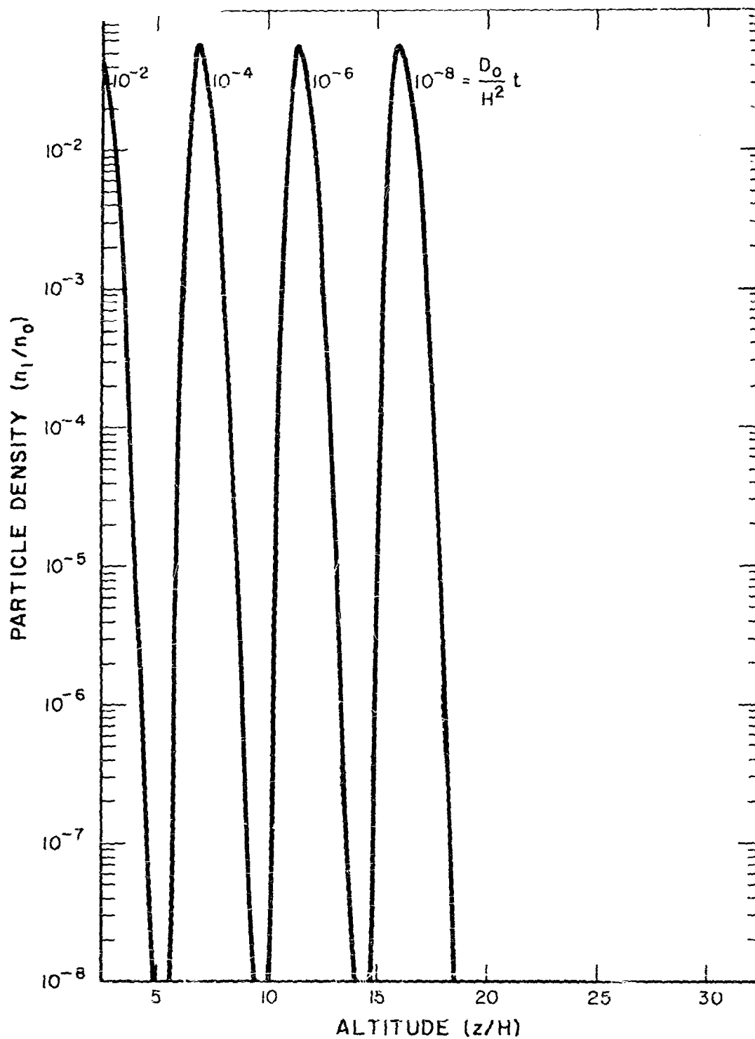
Figure 4. Particle density function \frac{n_1}{n_0} as a function of altitude for several values of time \frac{D_0}{H^2} t ; mass ratio \mu = 10 .
