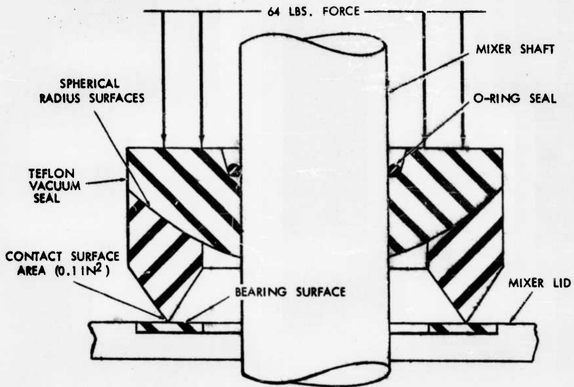
FIGURE 10 0814 Schematic Drawing of Self-Positioning Teflon Vacuum Seal for High Speed Mixing
