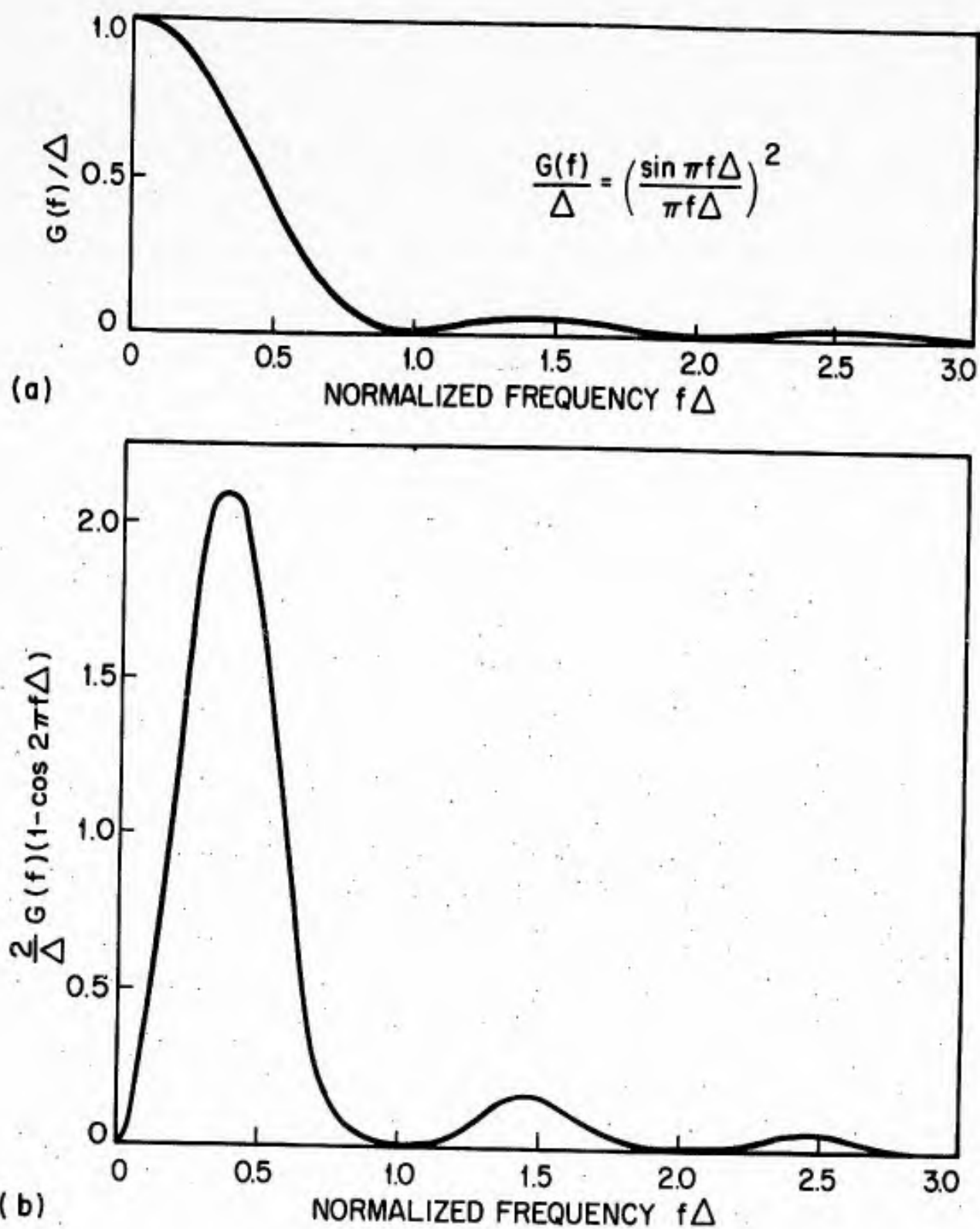
Fig. 3 "Envelopes" of power spectral densities, (a) binary sequence spectral density, (b) self-noise spectral density for \epsilon = \Delta
