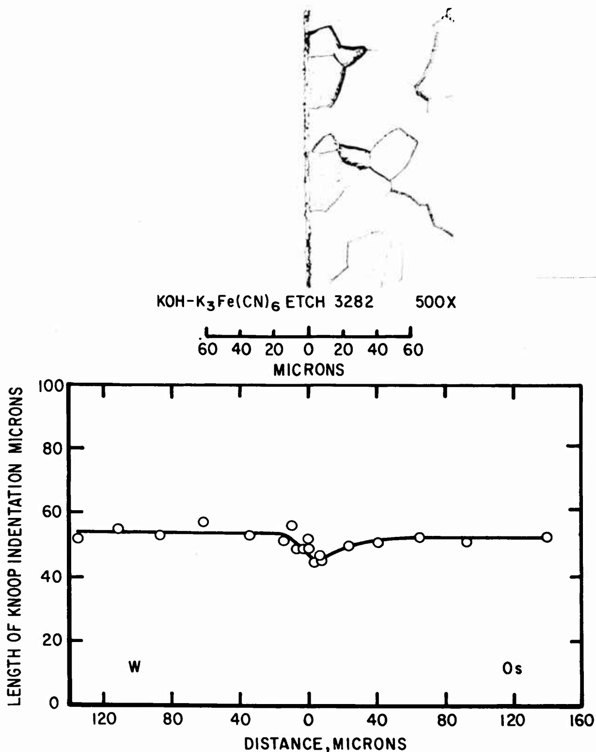
Fig.4-W-Os, pressure weld no.4a-4; microstructure and microindentation measurements of interdiffusion after annealing 4 hours at 1700°C.
