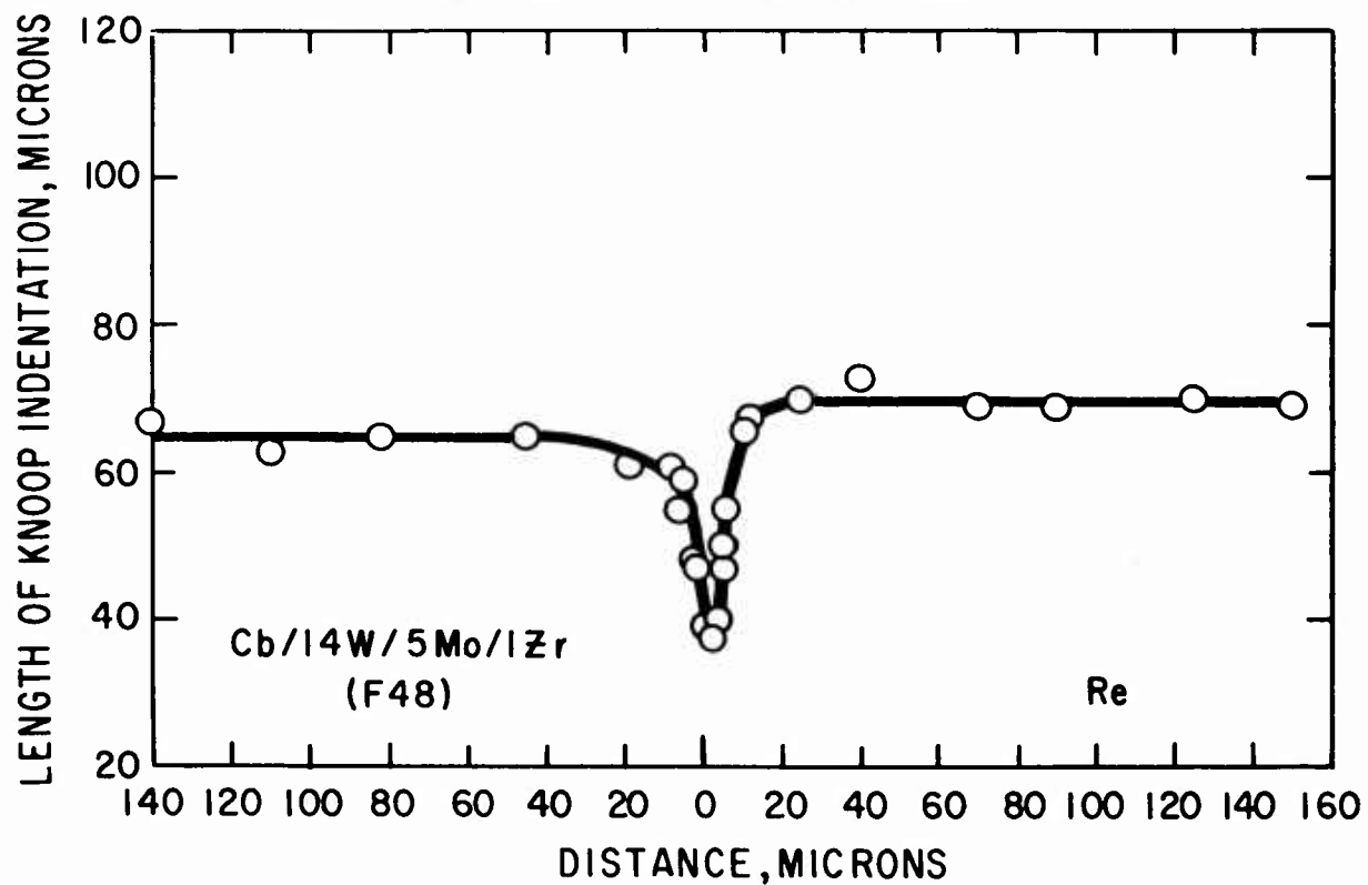
Fig.35- Cb (F48)- Re, pressure weld no.6c,annealed 4 hours at 1700°C
