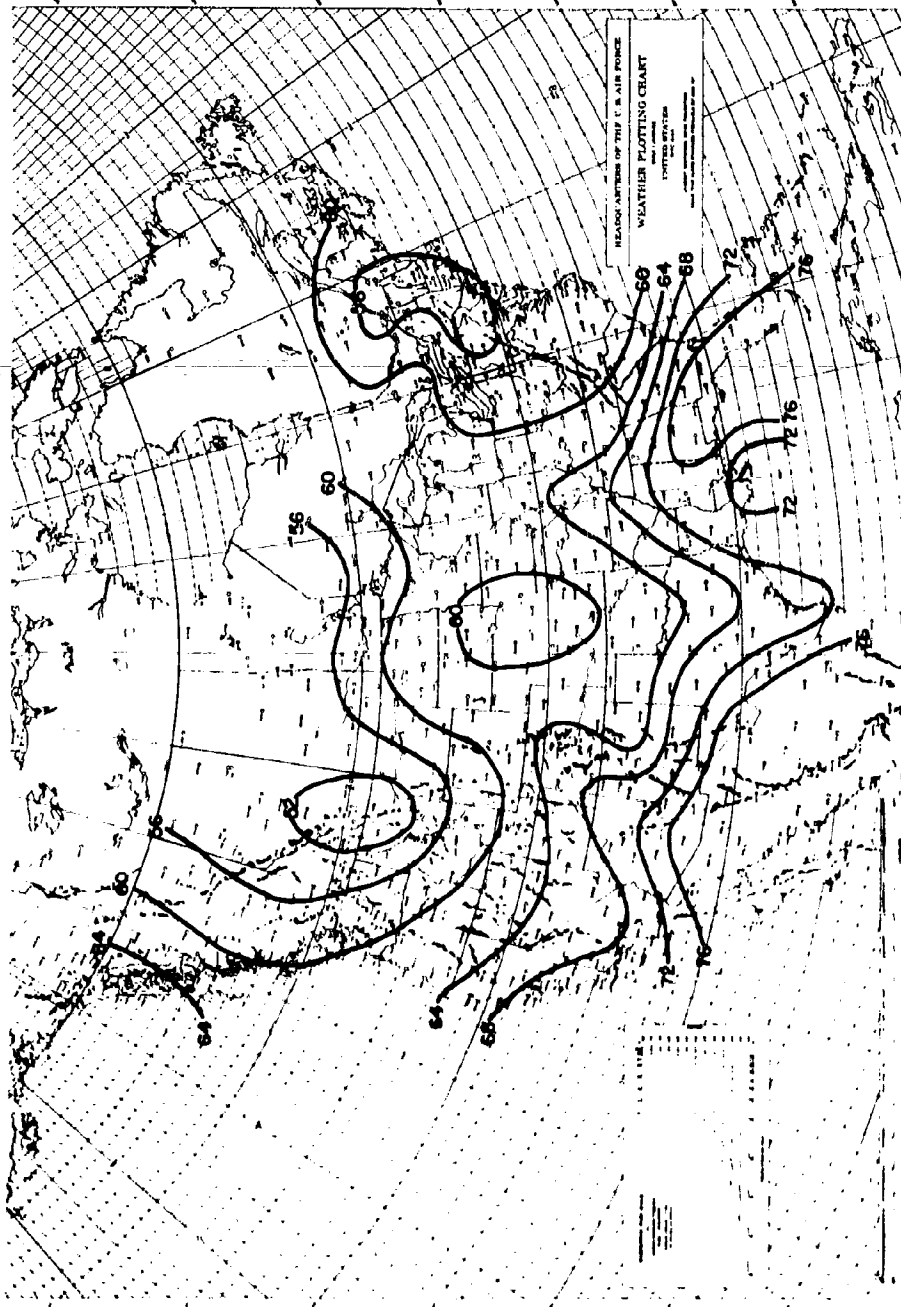
Figure 3. E.V.P. Percent (—) Reduction in Variance of Six-Hour Persistence Forecasts, Winter, 300mb.
