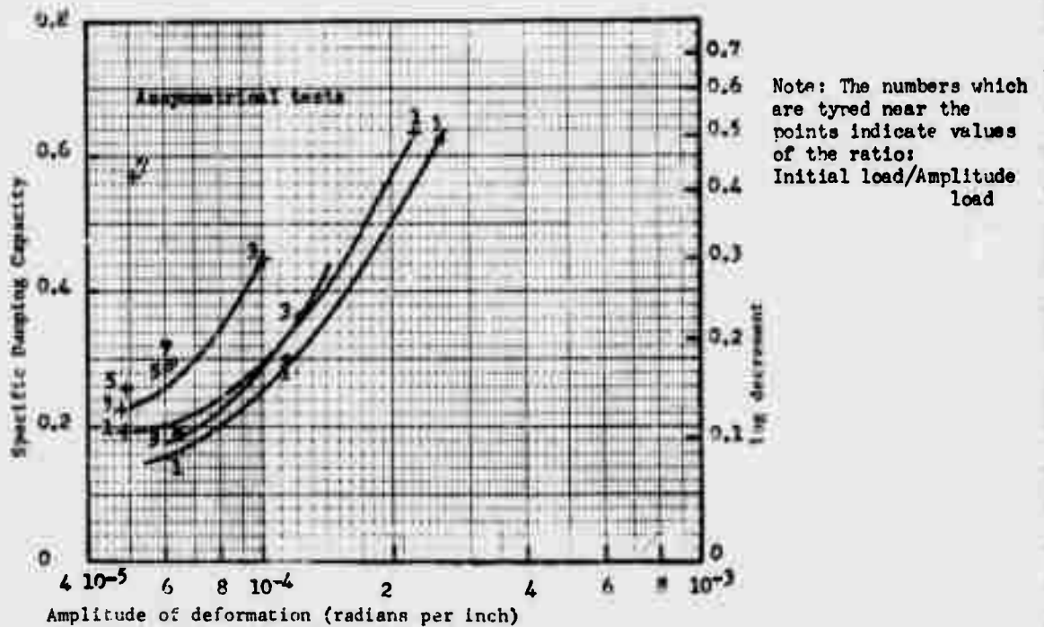
Fig. 4-7. - Relationship between damping and amplitude of deformation
