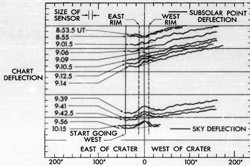
Fig. 36 Temperature Traces Over Aristarchus During Eclipse, September 5, 1960
