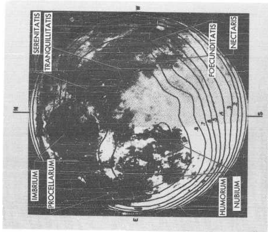
Fig. 15 Brightness Contours at 4.3 mm Wavelength 280° Lunar Phase
