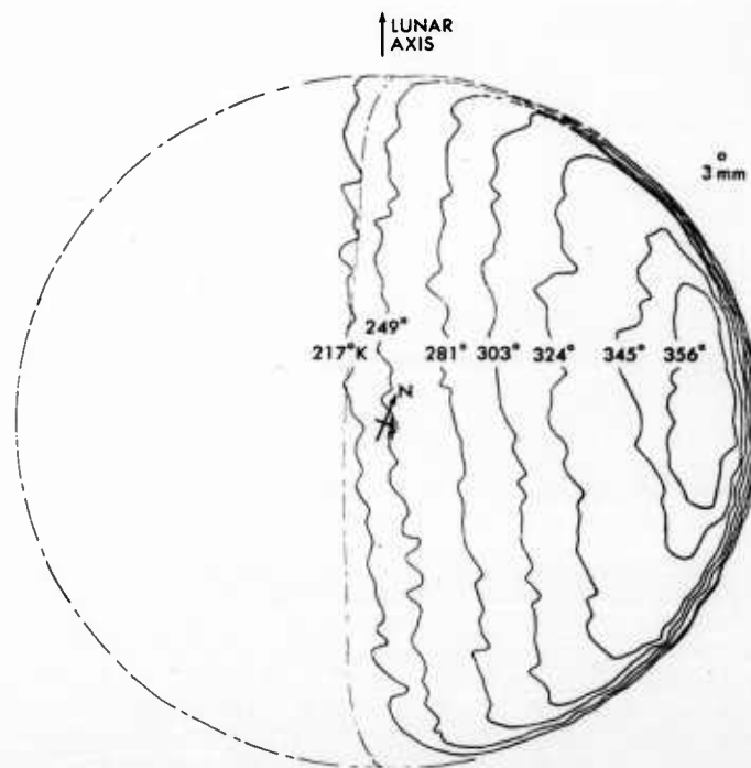
Fig. 4 Isothermal Contours of May 16, 1959 Start 1:49, End 4:43 UT, 58 Scans 0.53 Illuminated (~8 Day Old Moon)
