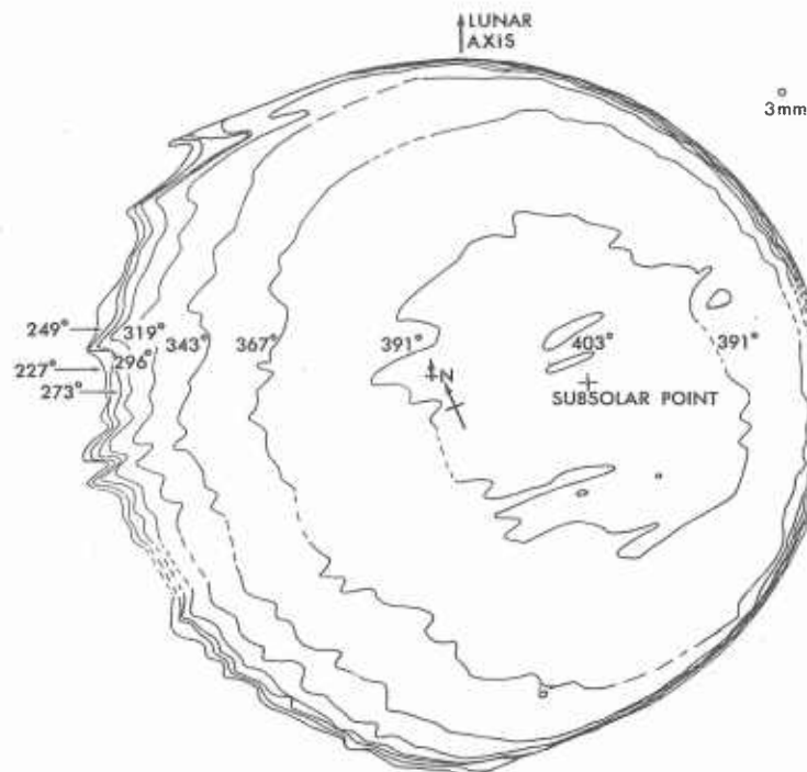
Fig. 6 Isothermal Contours of Setember 26, 1958, Start 3:55, End 7:01 UT, 63 Scans 0.98 Illuminated ( \sim 14 Day Old Moon)
