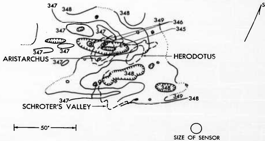
Fig. 28 Isotherms in the Region of Aristarchus Rectified to Remove the Effect of the Curvature of the Surface September 5, 1960, 6:57 UT
