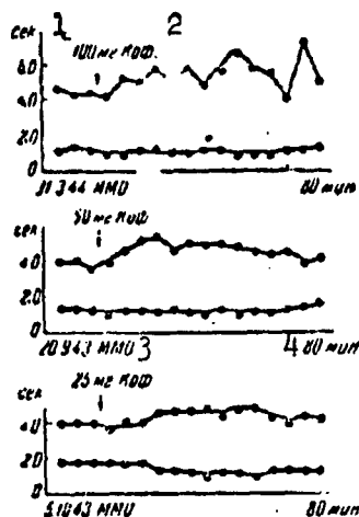
Fig. 3. Curves showing influence of caffeine on course of Purkinje afterimage. Other specifications same as for Fig. 2. 1) Sec; 2) mg. caffeine; 3) MMO; 4) min.
