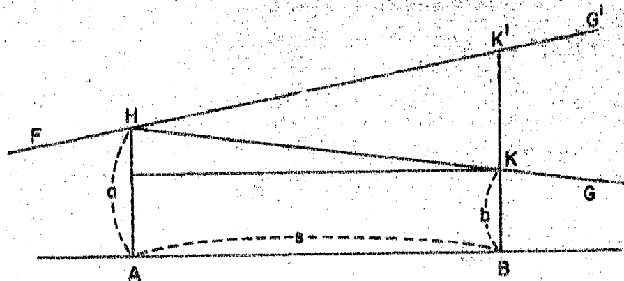
Figure 5. Situation on B's Unconditional Viability Boundary
