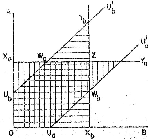
Figure 4. The Unconditional Viability Boundaries
