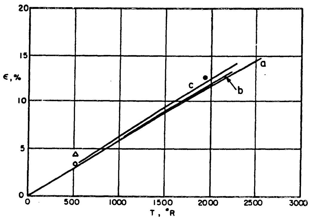
Fig. 15: Total Normal Emissivity of Platinum. Curve a, Abbott, (5) experimental; curve b, Equation 3.1, Abbott resistivity; curve c, same, handbook resistivity. Points correspond to Figure 13.
