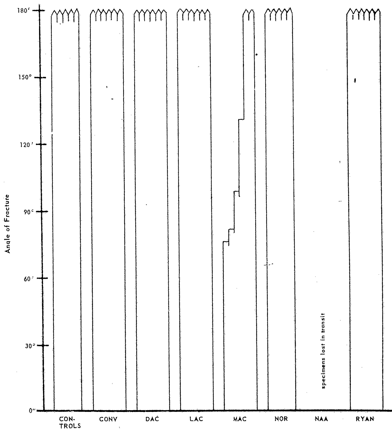
Graph 5, Phase I Constant-Rate Bend Test Results (Norair)
