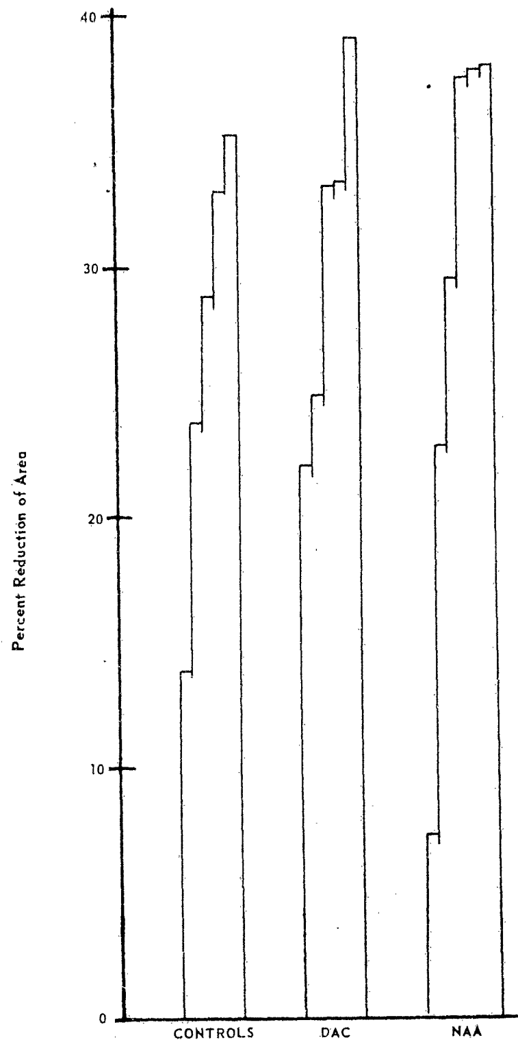
Graph 7. Phase II Constant-Strain-Rate Tensile Test Results (Convair)
