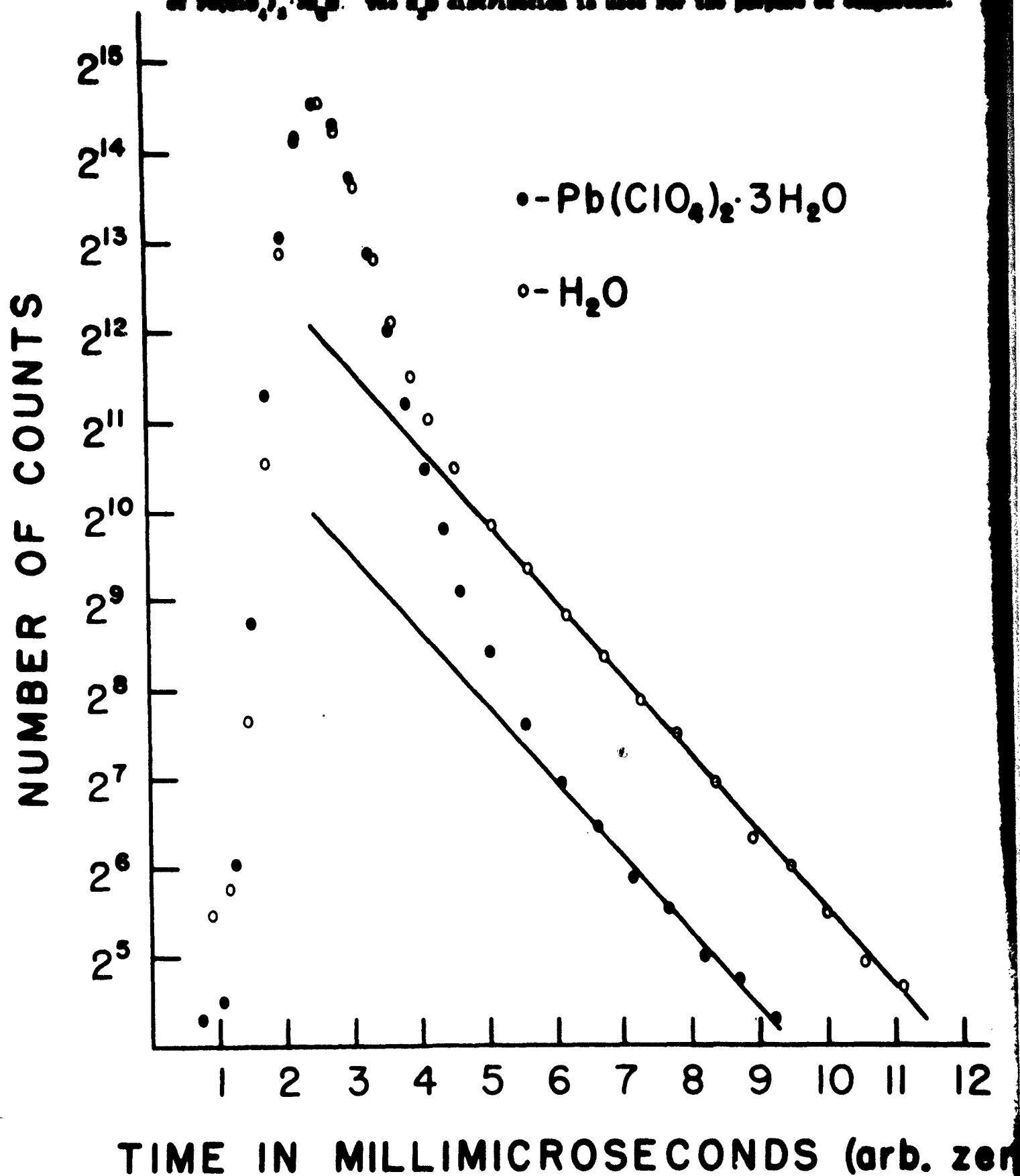
Fig. 4. Time distribution of positron annihilations in an aqueous solution of \text{Pb}(\text{ClO}_4)_2 \cdot 3\text{H}_2\text{O} . The \text{H}_2\text{O} distribution is used for the purpose of comparison.
