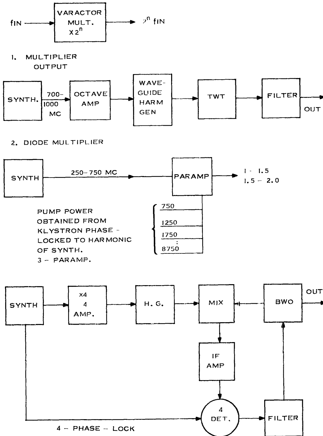
Fig. 6-1 Harmonic Generators
