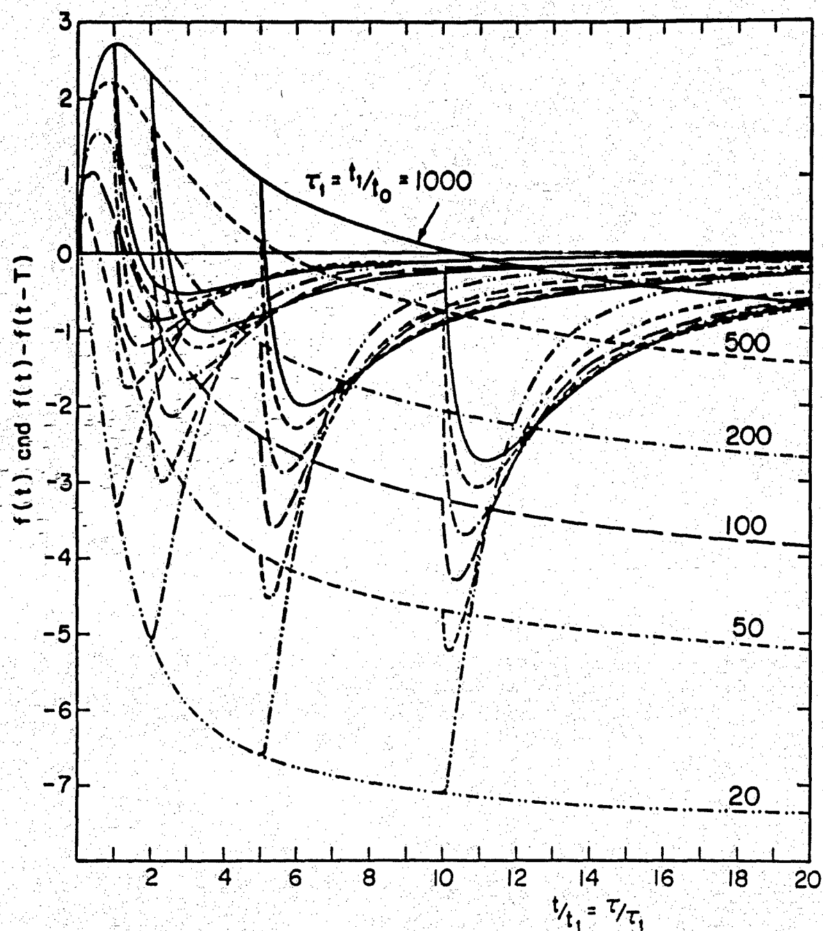
FIG. 8 SUPERPOSITION OF THE CURVES OF FIG. 7
