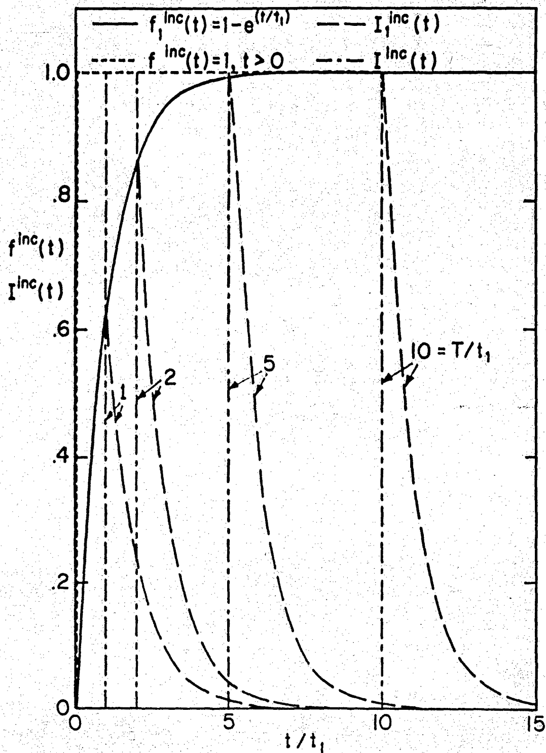
FIG. 4 INCIDENT STEP AND PULSE WITH INFINITE AND FINITE RISE TIME t_1 , AND PULSE LENGTH T
