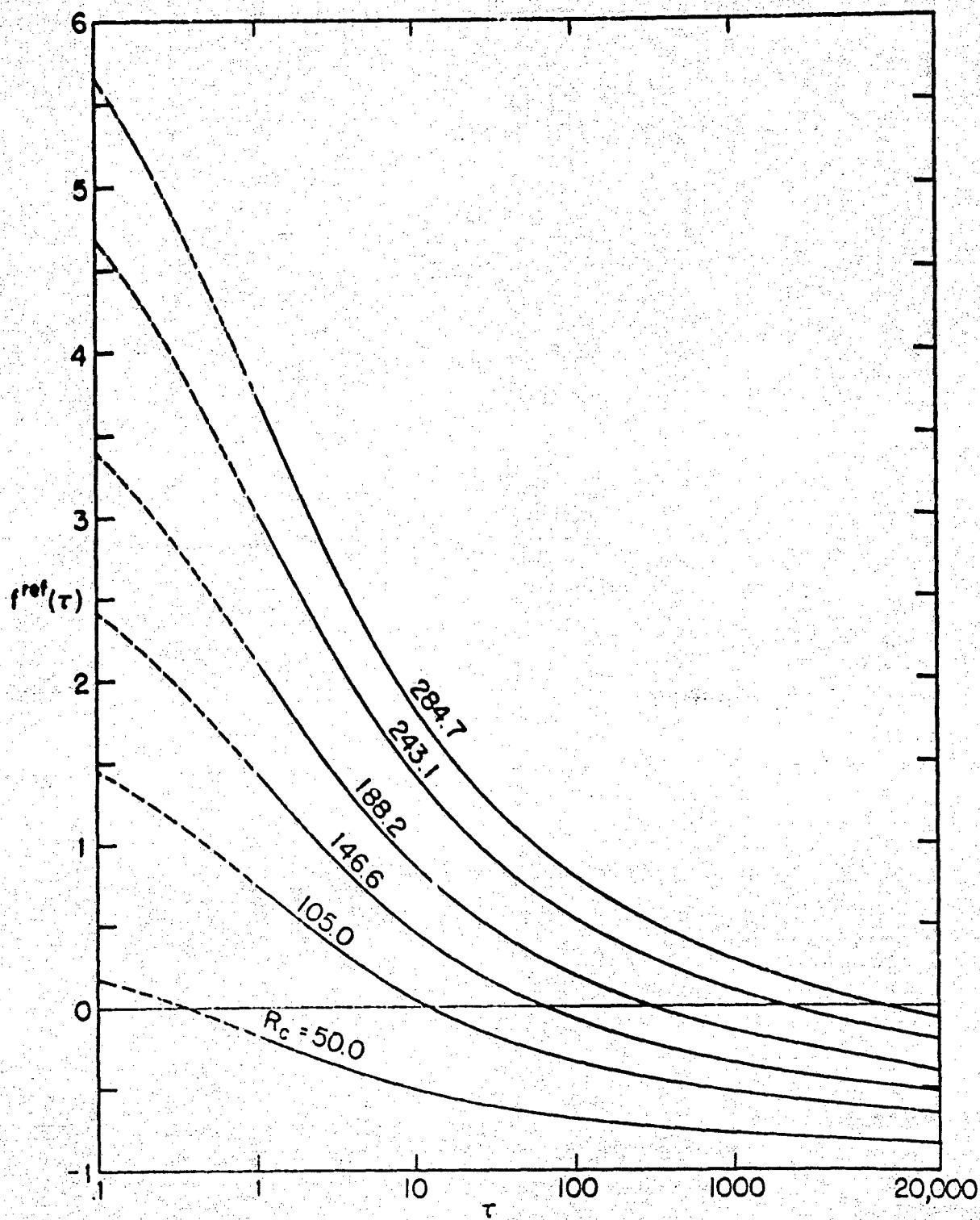
FIG. 5 REFLECTION f^{\text{ref}}(\tau) OF INCIDENT SHARP STEP. \tau = t/t_0
