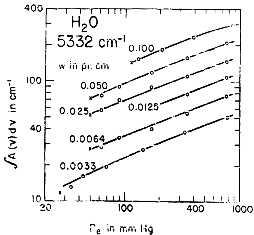
Fig. 10. The total absorption of the 5332 \text{ H}_2\text{O} band versus P_e . The x points correspond to samples of \text{H}_2\text{O} alone, the circle points to samples of \text{H}_2\text{O} and \text{N}_2 .
