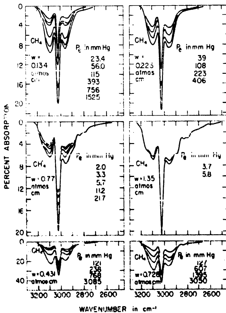
Fig. 44. Spectra of the 3000 cm -1 CH 4 band
