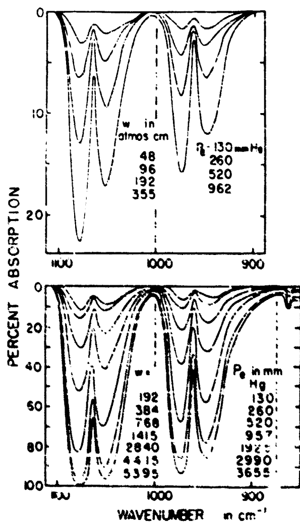
Fig. 16. Absorption curves of the 10 \mu and 9 \mu CO 2 bands. The ordinate scale of the spectrometer was extended by a factor of 5 while obtaining spectra shown in the upper portion of the figure.
