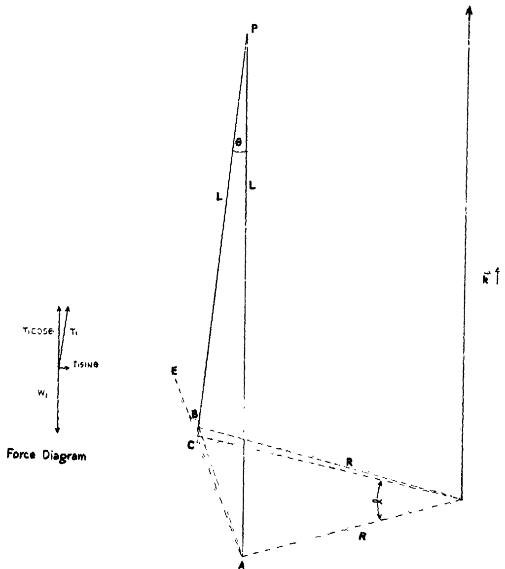
Figure 14. Schematic Diagram for One Wire When Pendulum Bob is Turned an Angle \gamma
