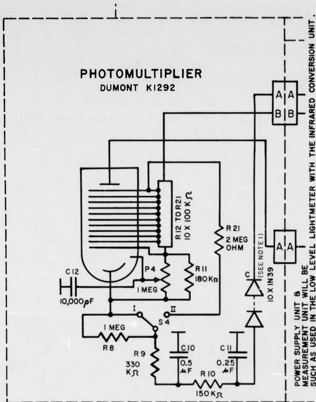
Figure 1. Schematic Diagram for Low-Level Lightmeter for the Near-Infrared
