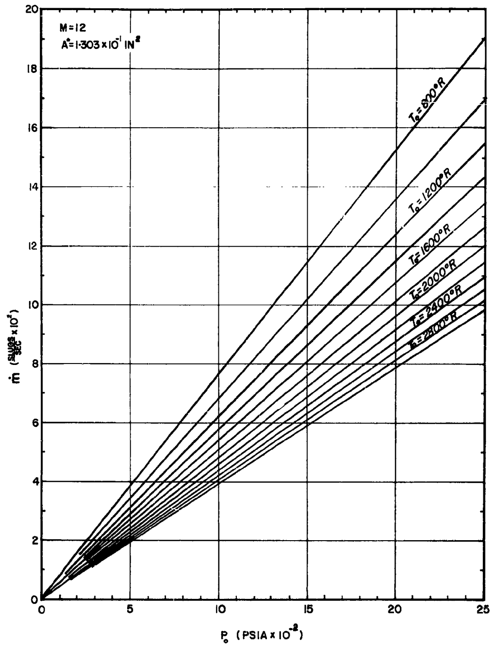
FIG. 11c MASS FLOW RATE vs. STAGNATION PRESSURE.
