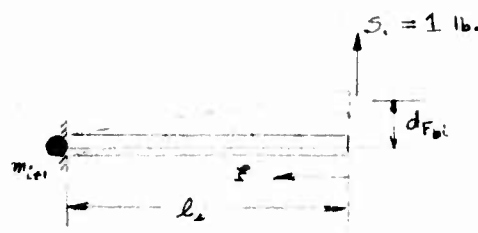
3b SHEAR EFFECT
