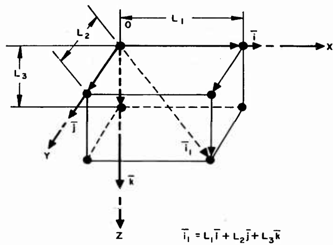
Figure 31. Direction Cosines
