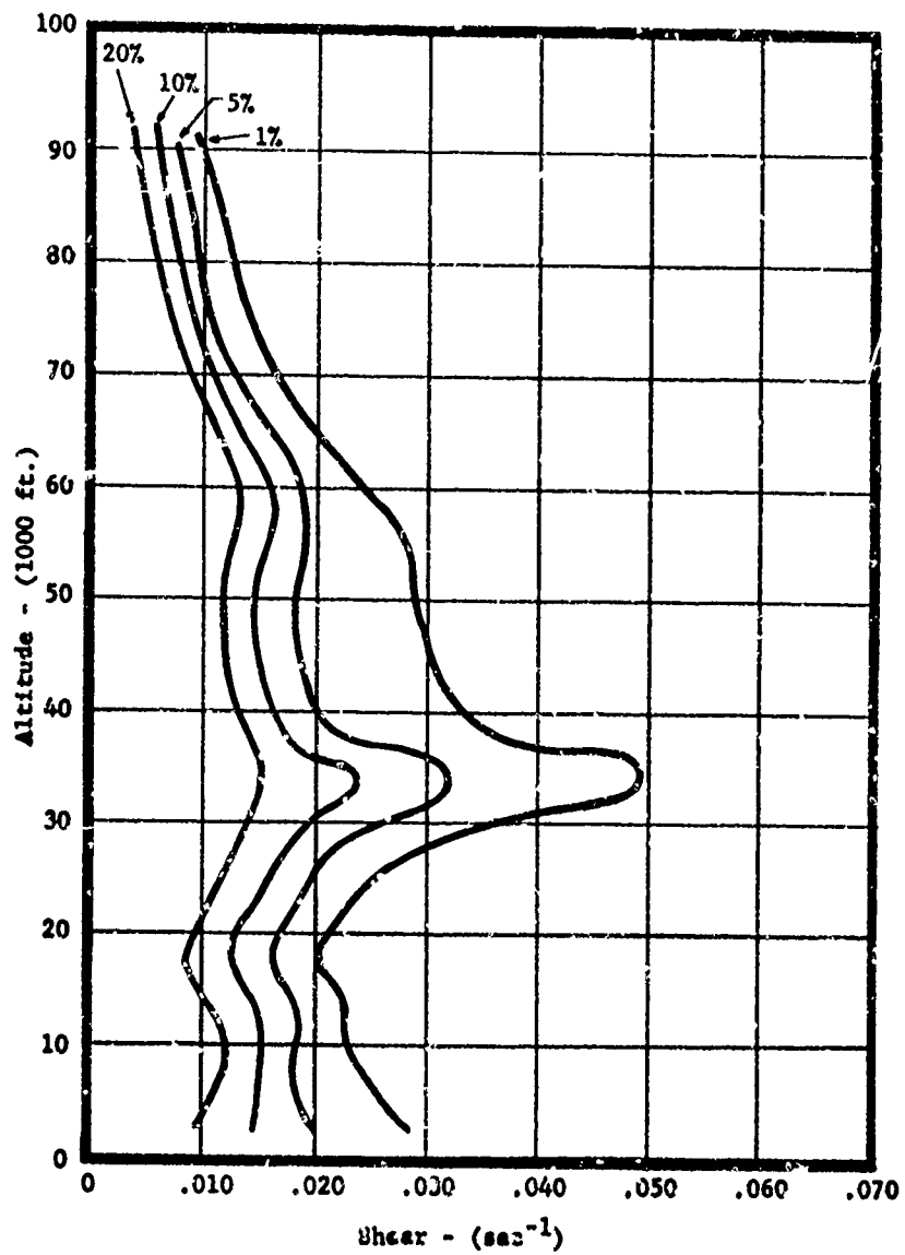
Figure 18. Probability of Occurrence with Height of Extreme 3,000 foot Longitudinal Shear.
