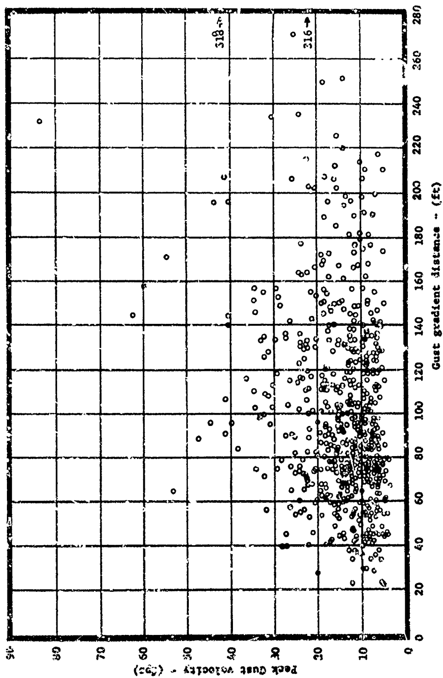
Figure 24. Gust Velocity as a Function of Gust-Gradient Distance.
