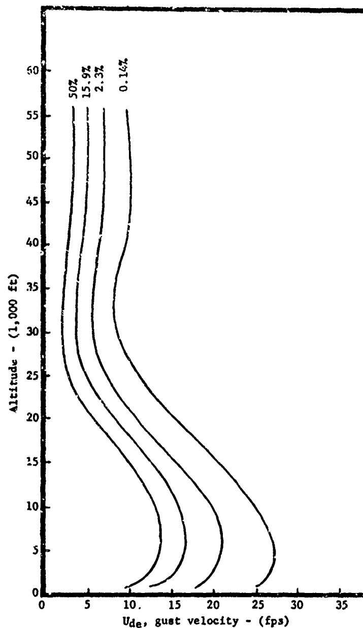
Figure 25. Nonthunderstorm Gust Probability of Occurrence.
