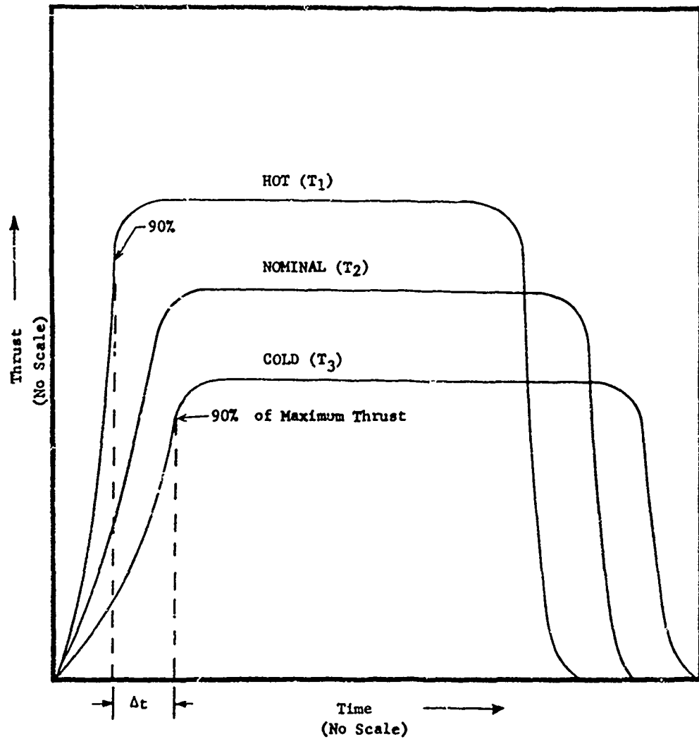
Figure 32. Thrust Characteristics for Solid Propellant Motors for Various Propellant Temperatures
