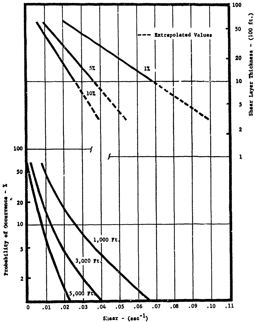
Figure 15. Probability of Occurrence and Layer Thickness for Longitudinal Shears at Level of Strongest Winds.
