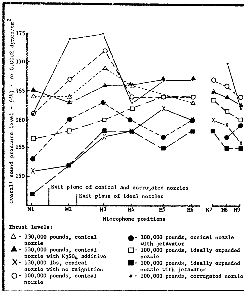
Figure 41a. Average Overall Near Field Sound Pressure Levels.
