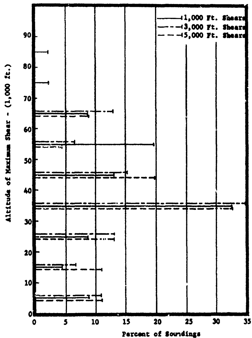
Figure 16. Percent Altitude Occurrence of Maximum 1,000, 3,000, and 5,000-foot Longitudinal Shears.
