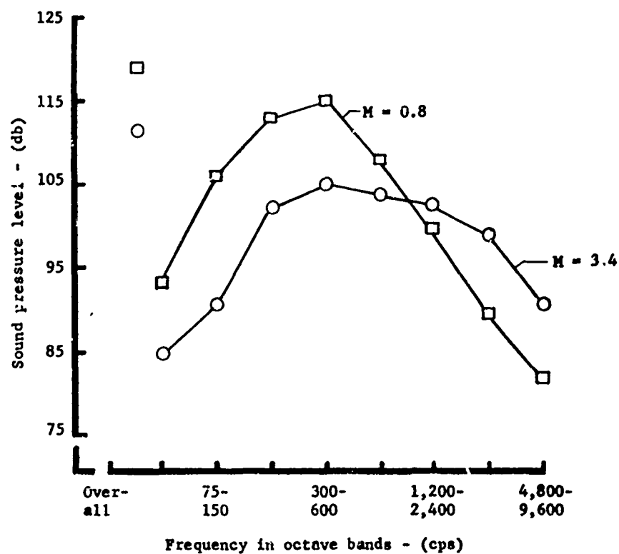
Figure 37. Internal Sound Spectra at Constant q for Various Mach Numbers
