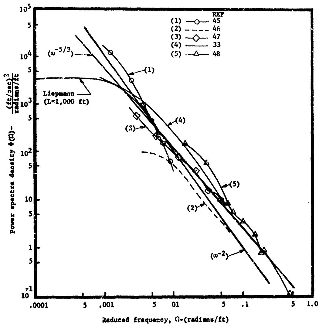
Figure 28. Analytical and Measured Gust Power Spectra Data
