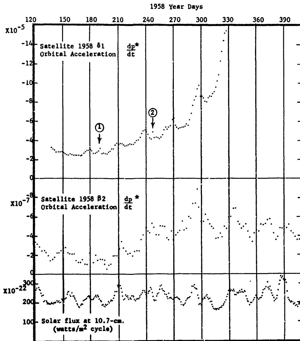
Figure 51. Secular Acceleration of Satellites 1958 Delta I and 1958 Beta II Compared to 10.7-cm Solar Flux
