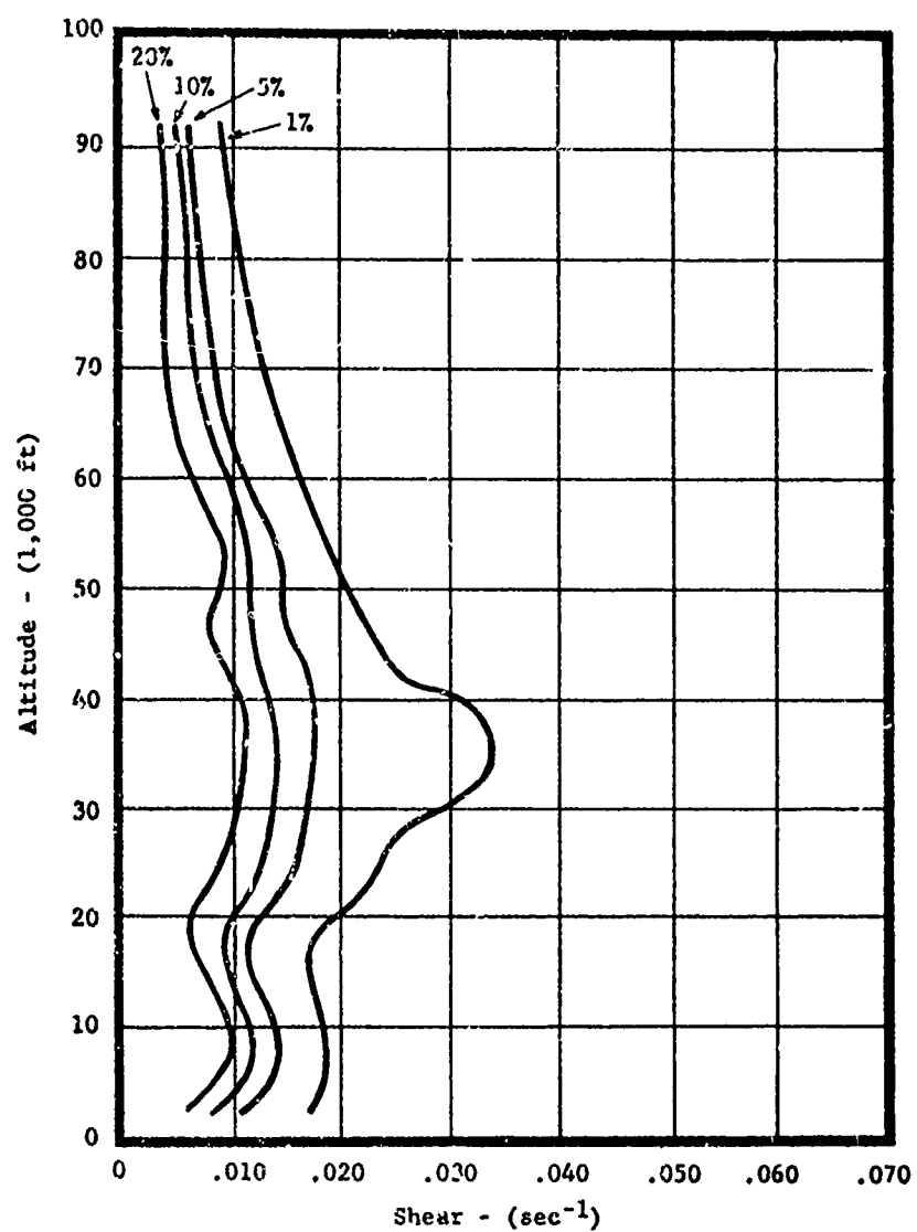
Figure 19. Probability of Occurrence with Height of Extreme 5,000 foot Longitudinal Shear.
