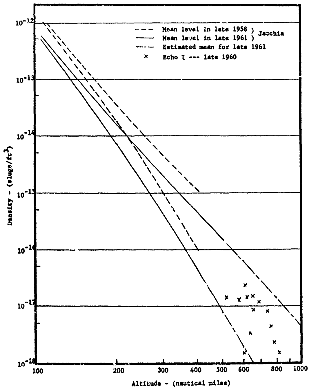
Figure 54b. Atmospheric Density
