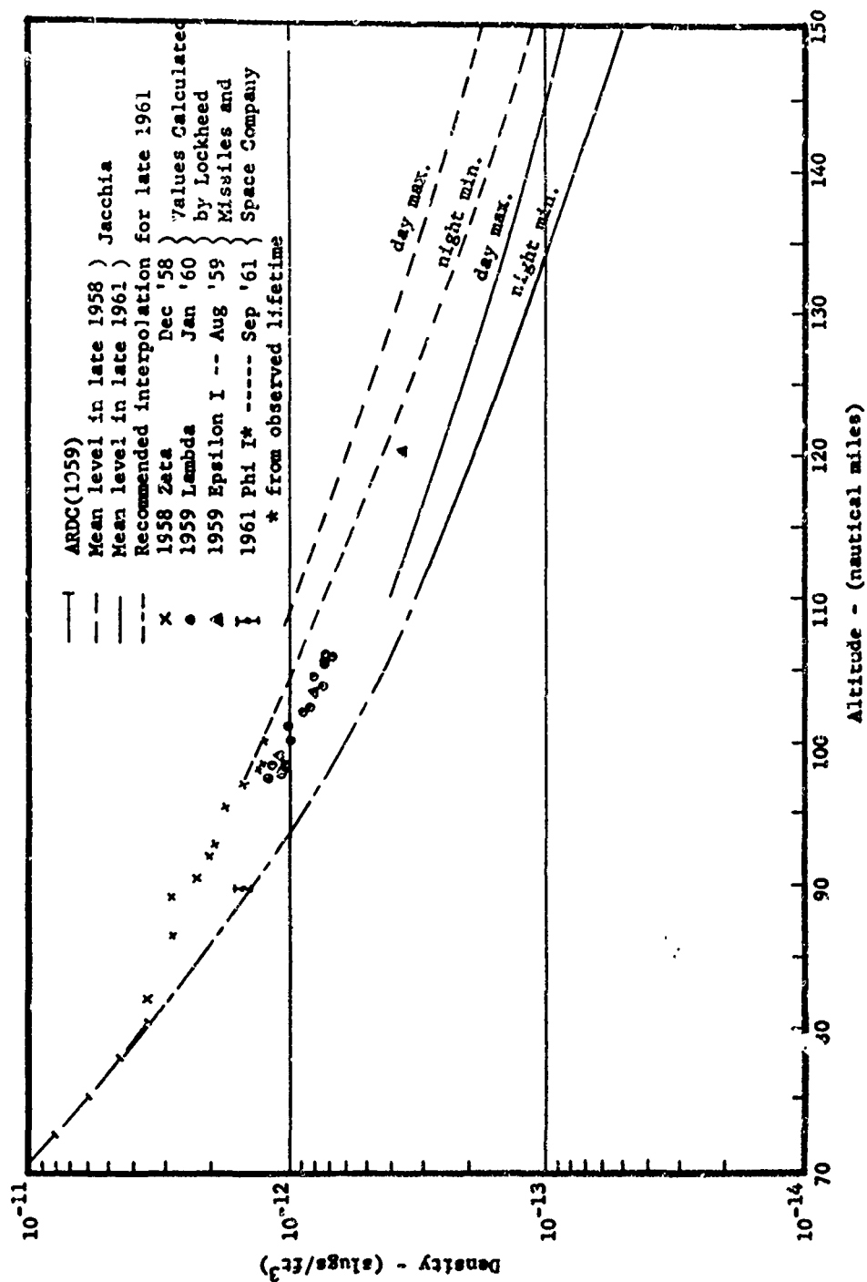
Figure 54a. Atmospheric Density
