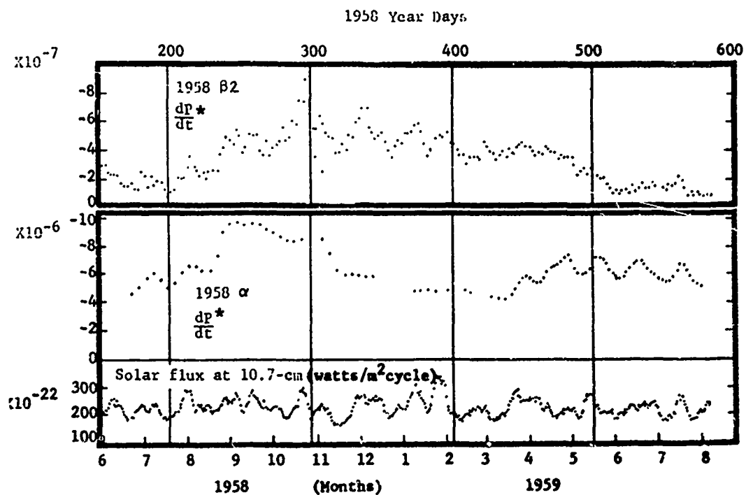
Figure 52. Secular Acceleration of Satellites 1958 Beta II and 1958 Alpha, Compared with 10.7-cm Solar Flux.
