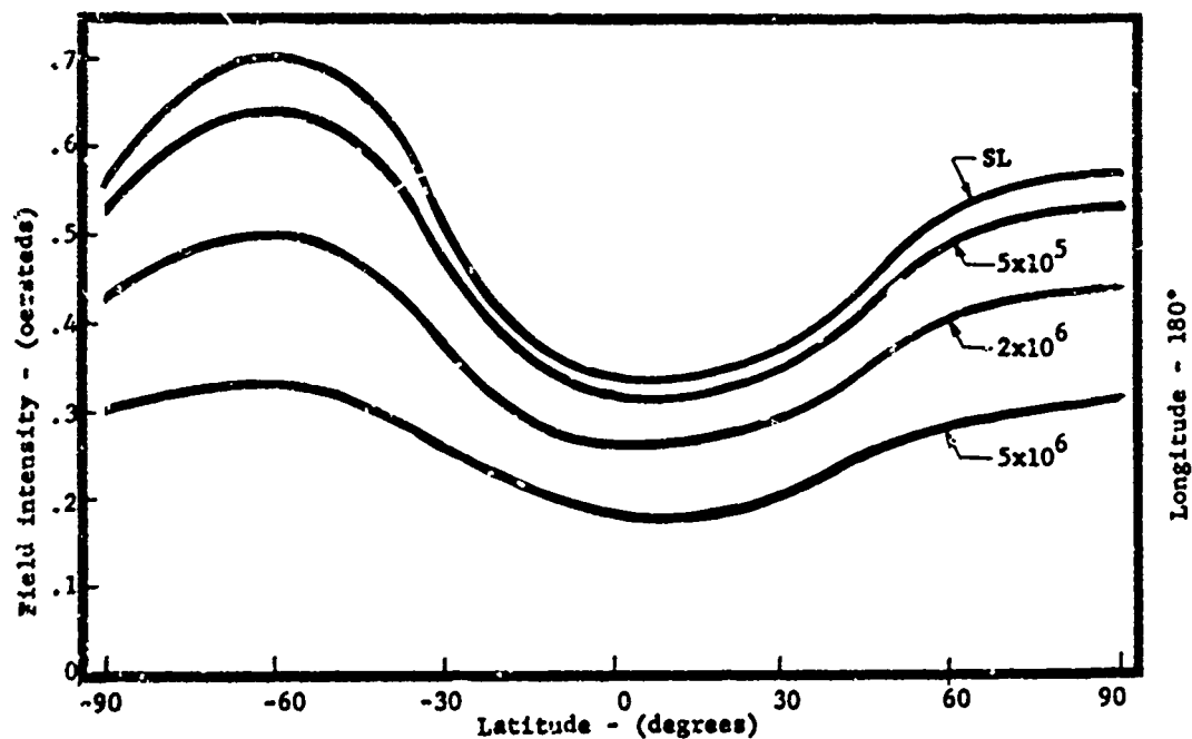
Figures 47 and 48. Magnetic Field Intensity at 120° and 180° Longitude
