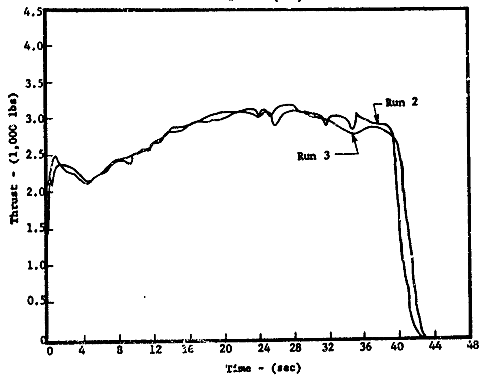
Figure 34. Thrust-Time Curves Comparison
