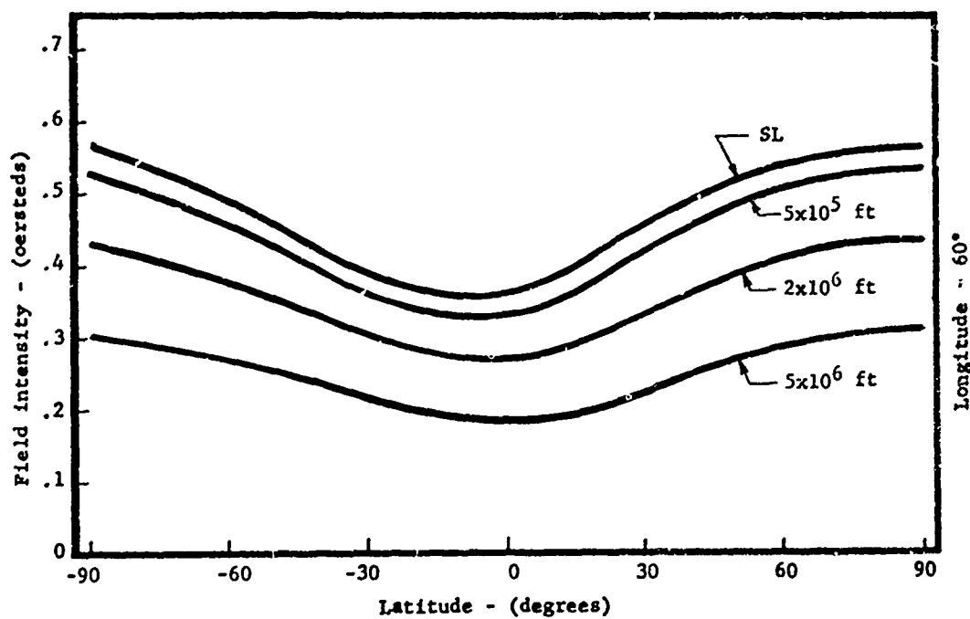
Figures 45 and 46, Magnetic Field Intensity at 0° and 60° Longitude
