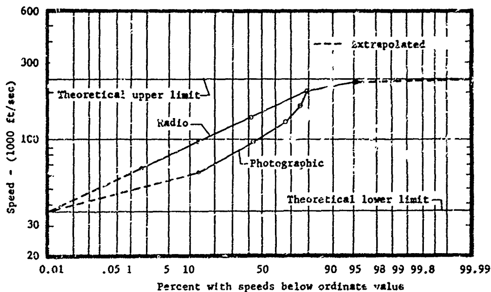
Figure 56. Distribution of Geocentric Meteor Speeds
