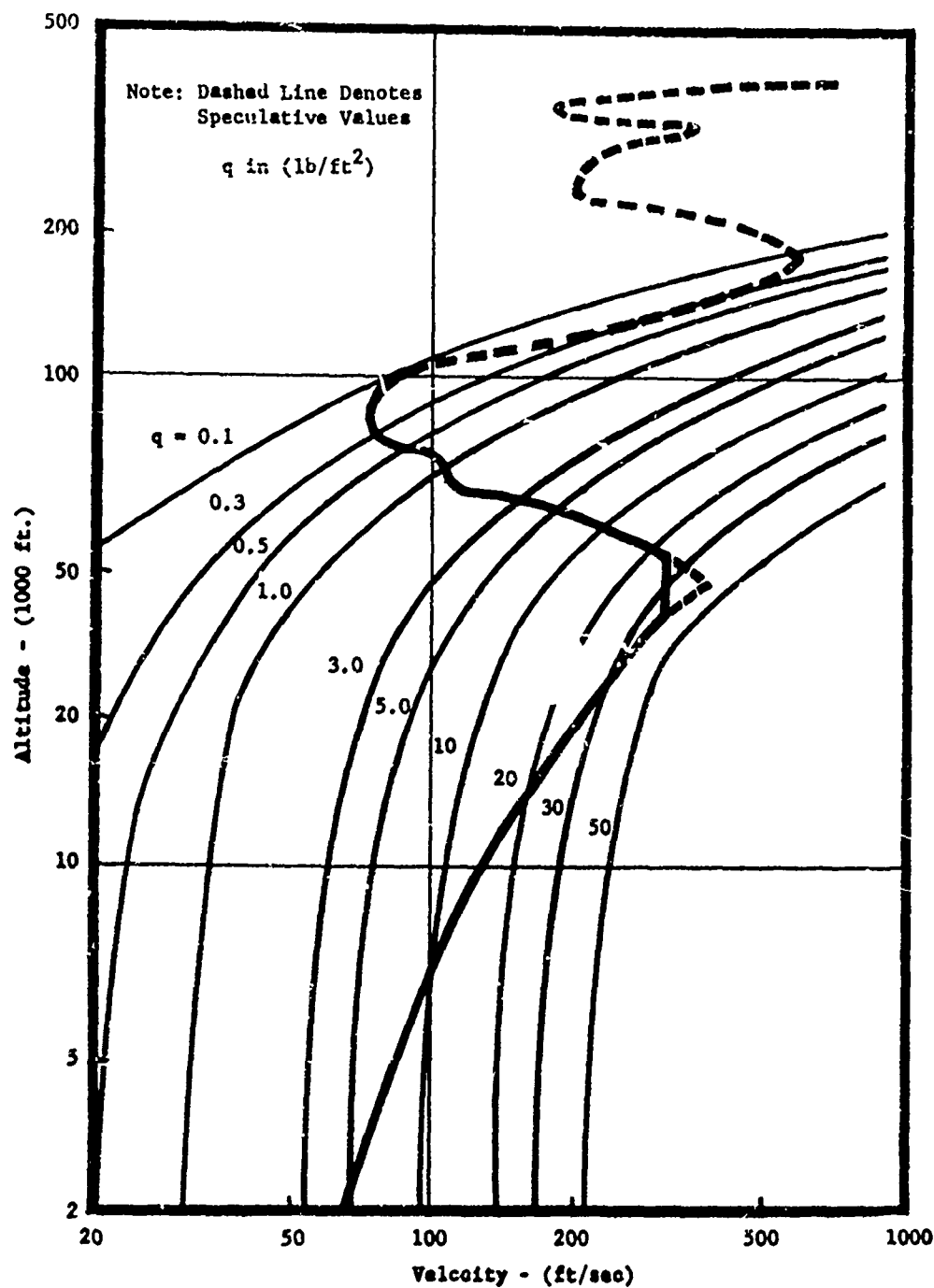
Figure 3. 1% Wind Speed Profile as Related to Altitude & q
