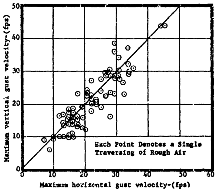
Figure 20. Horizontal and Vertical Gust Relationship
