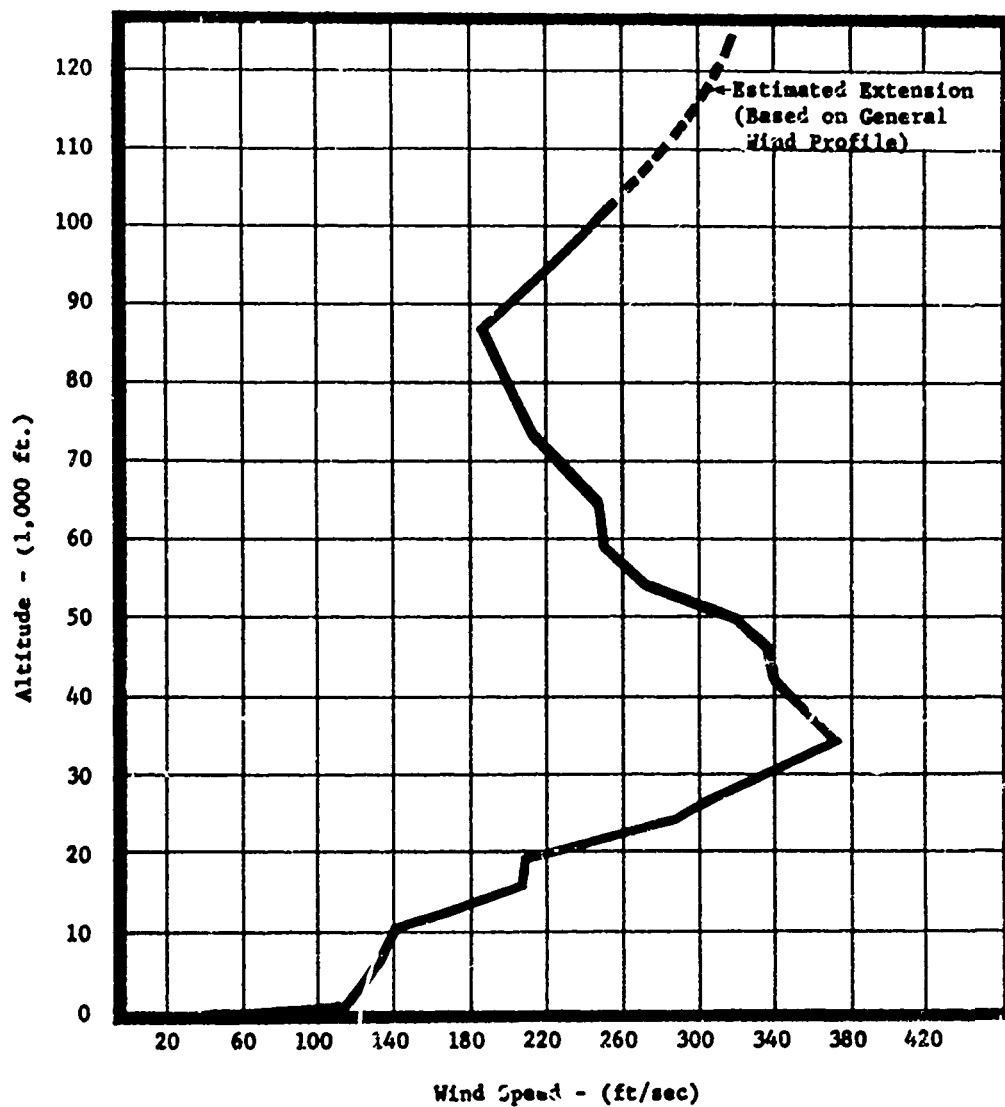
Figure 11.. Wind Speed Profile for 0.1% Probability
