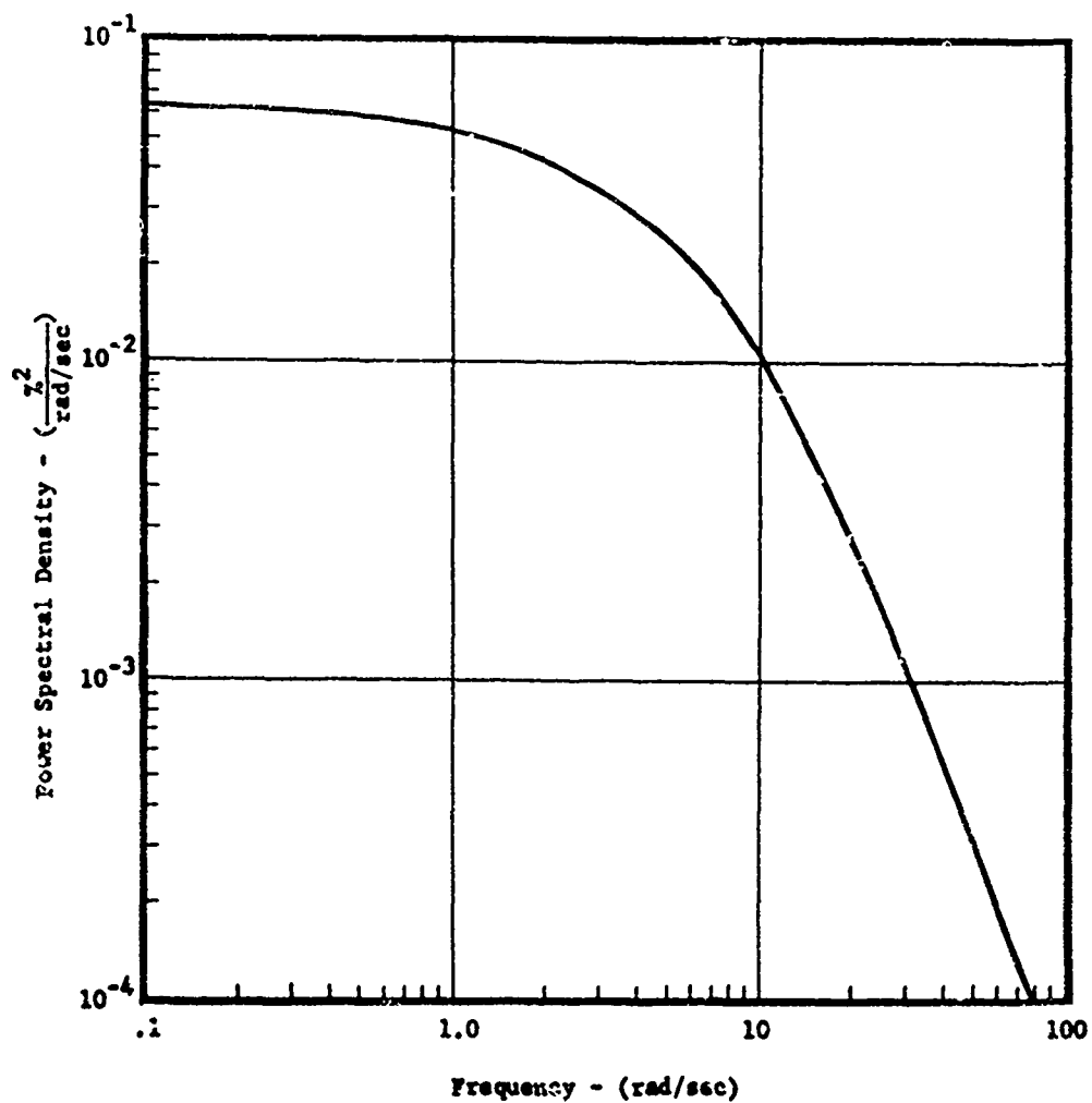
Figure 33. Thrust Percent Variation Power Spectrum
