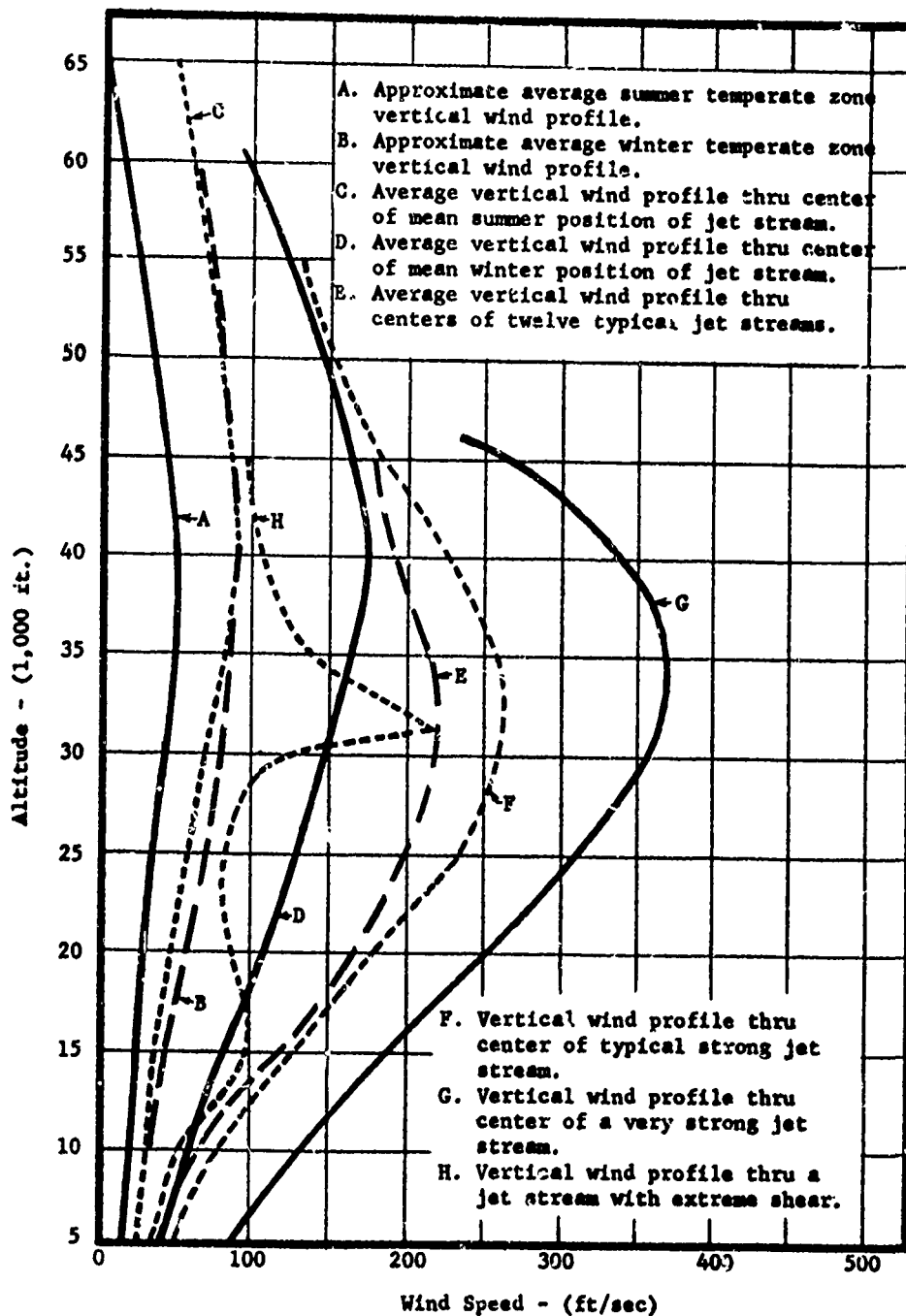
Figure 5. Typical Wind Speed Profiles
