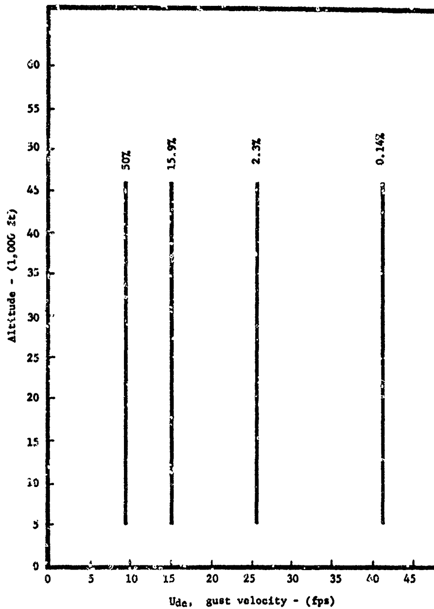
Figure 20. Thunderstorm Gust Probability of Occurrence.
