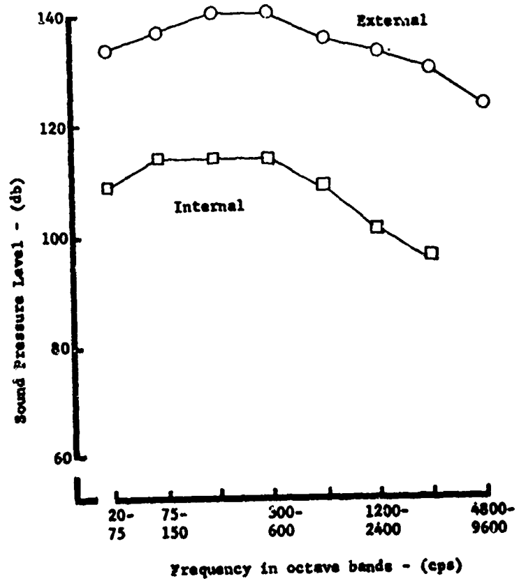
Figure 36. Nose Cone Noise from Rocket Engines
