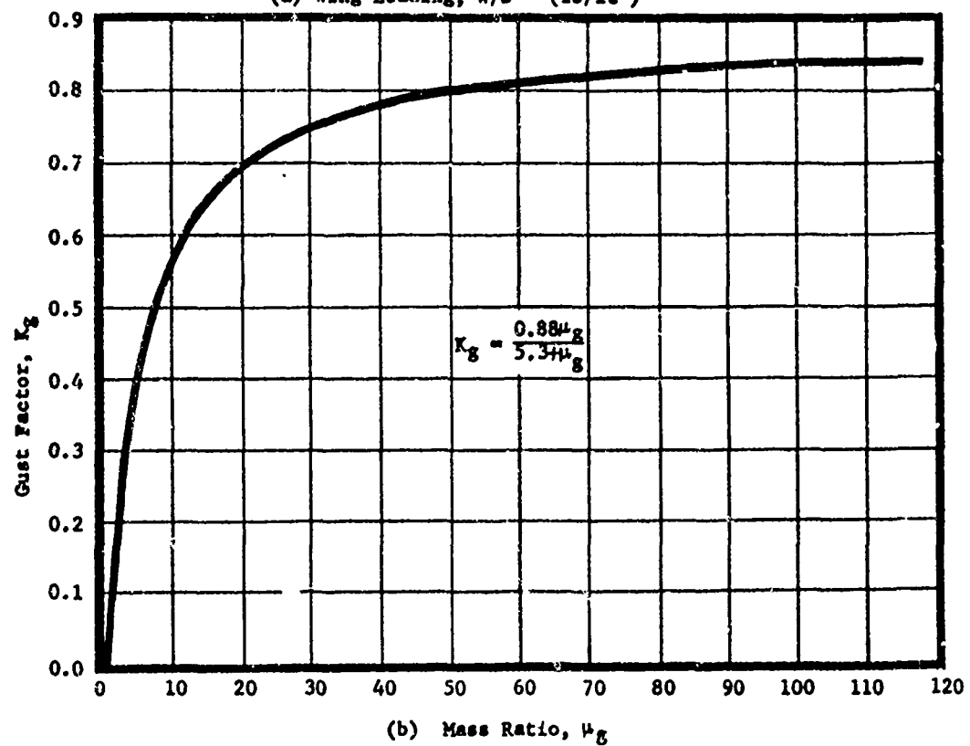
Figure 21. Gust Factors
