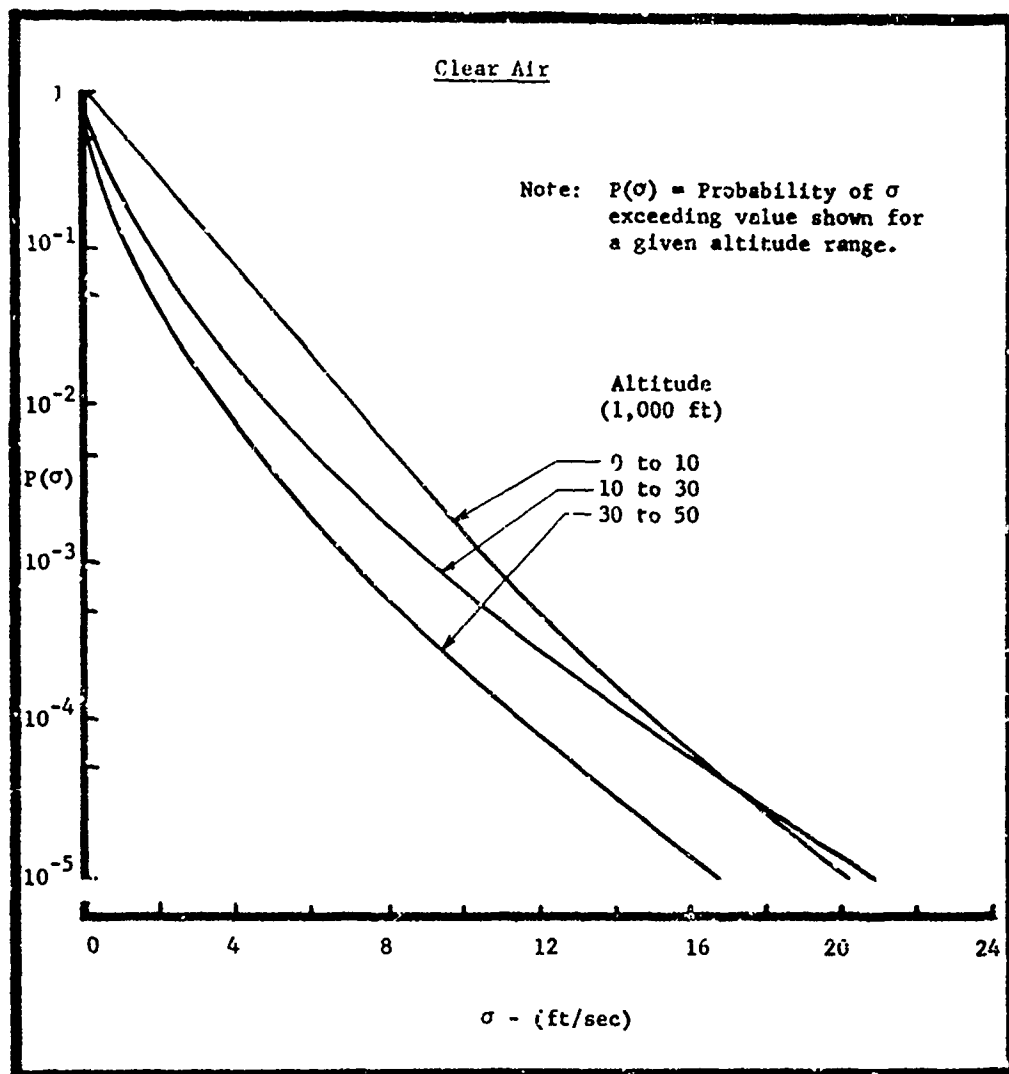
Figure 29. Cumulative Probability Distributions of Root-Mean-Square Gust Velocity
