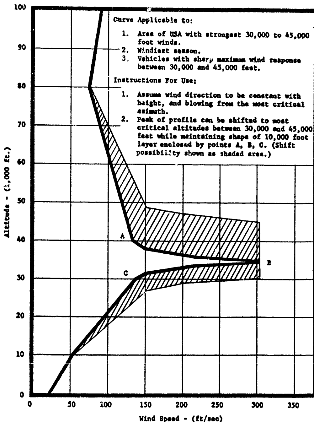
Figure 10. Synthetic Wind Speed Profile for 1% Probability
