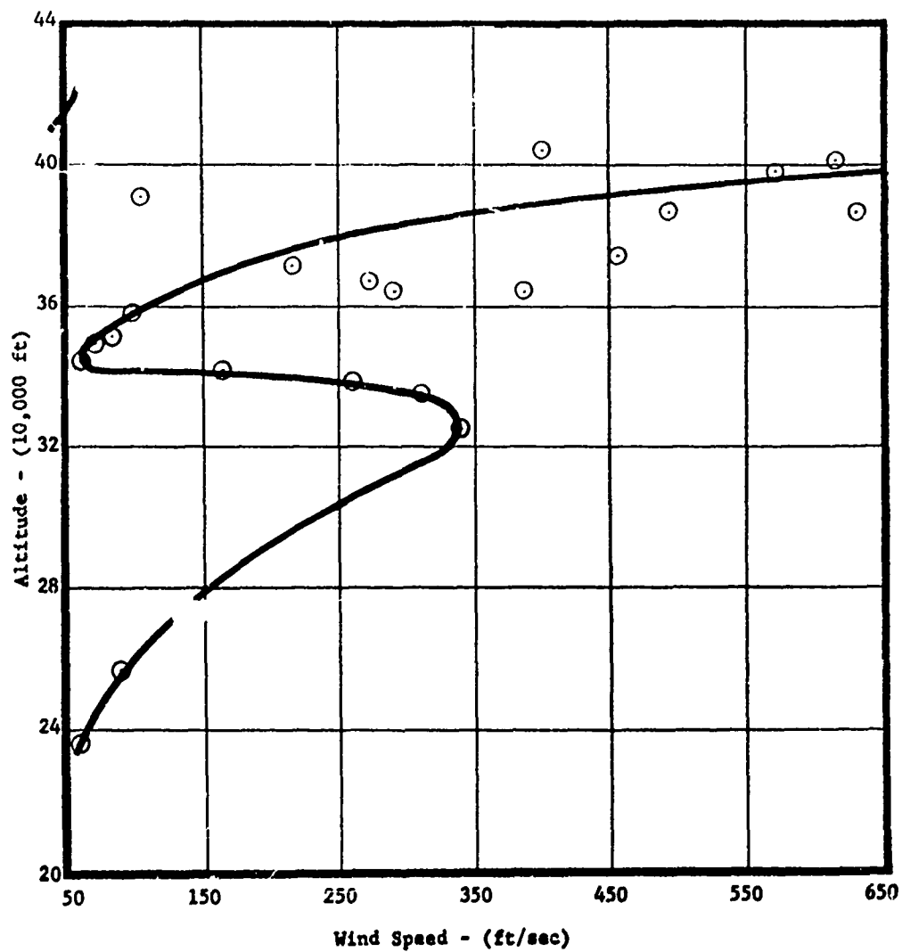
Figure 8. Wind Speed Profile for Upper Atmosphere Extremes
