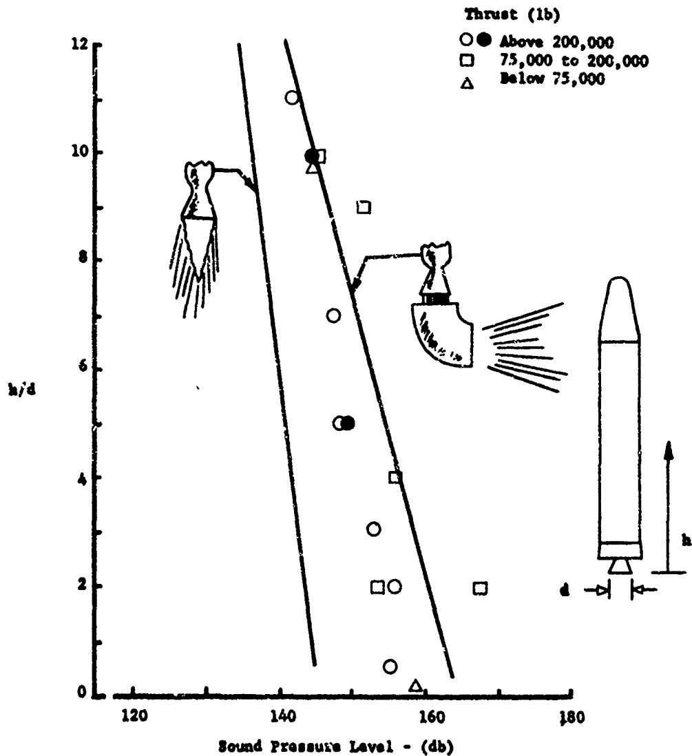
Figure 35. External Sound Pressure Levels at Lift-Off.
