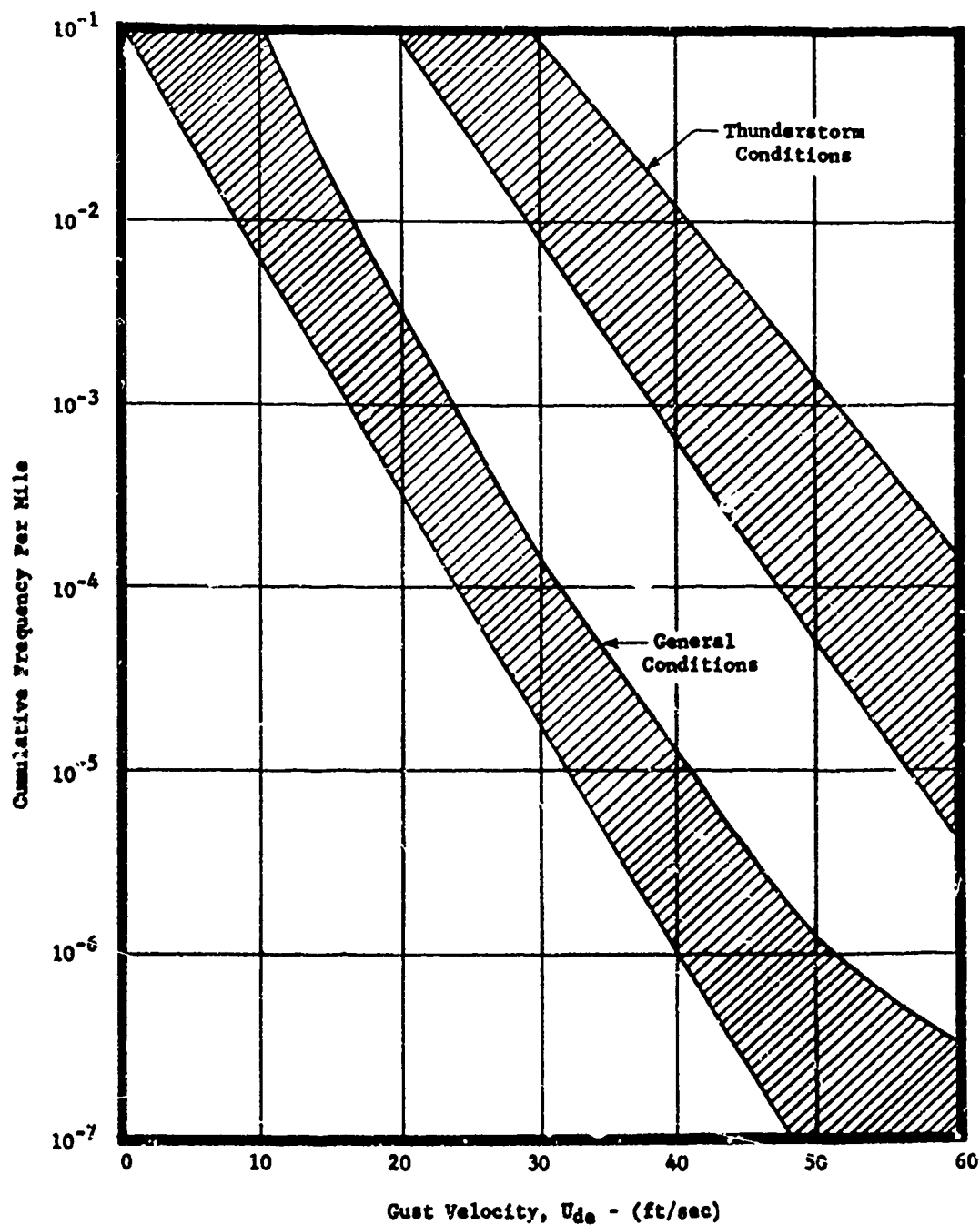
Figure 22. Cumulative Gust Frequency Per Mile of Flight.
