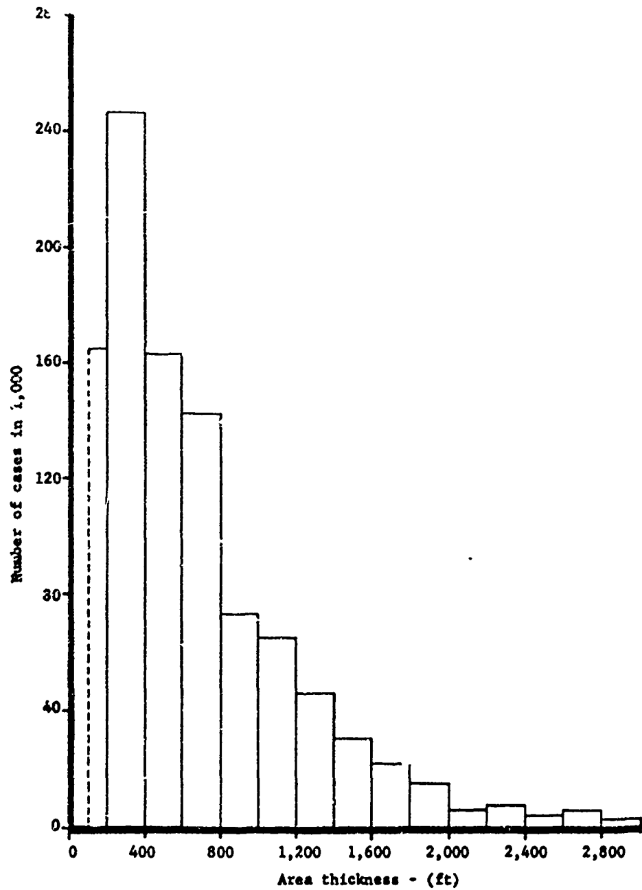
Figure 23. Variation in Thickness for Area of Norththunderstorm Turbulence
