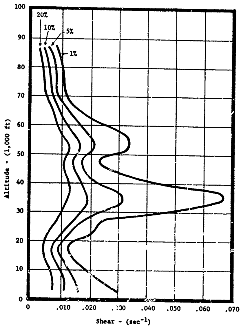
Figure 17. Probability of Occurrence with Height of Extreme 1,000 foot Longitudinal Shear.
