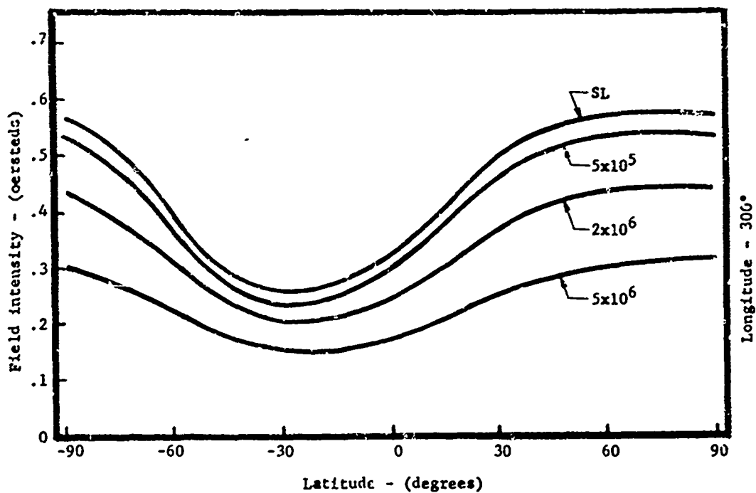
Figures 49 and 50. Magnetic Field Intensity at 240° and 300° Longitude
