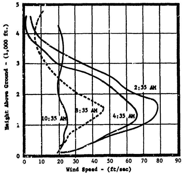
Figure 7. A Typical Low Level Jet Stream
