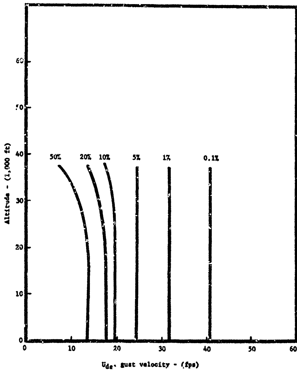
Figure 27. Average Gust Velocity Probability of Occurrence.
