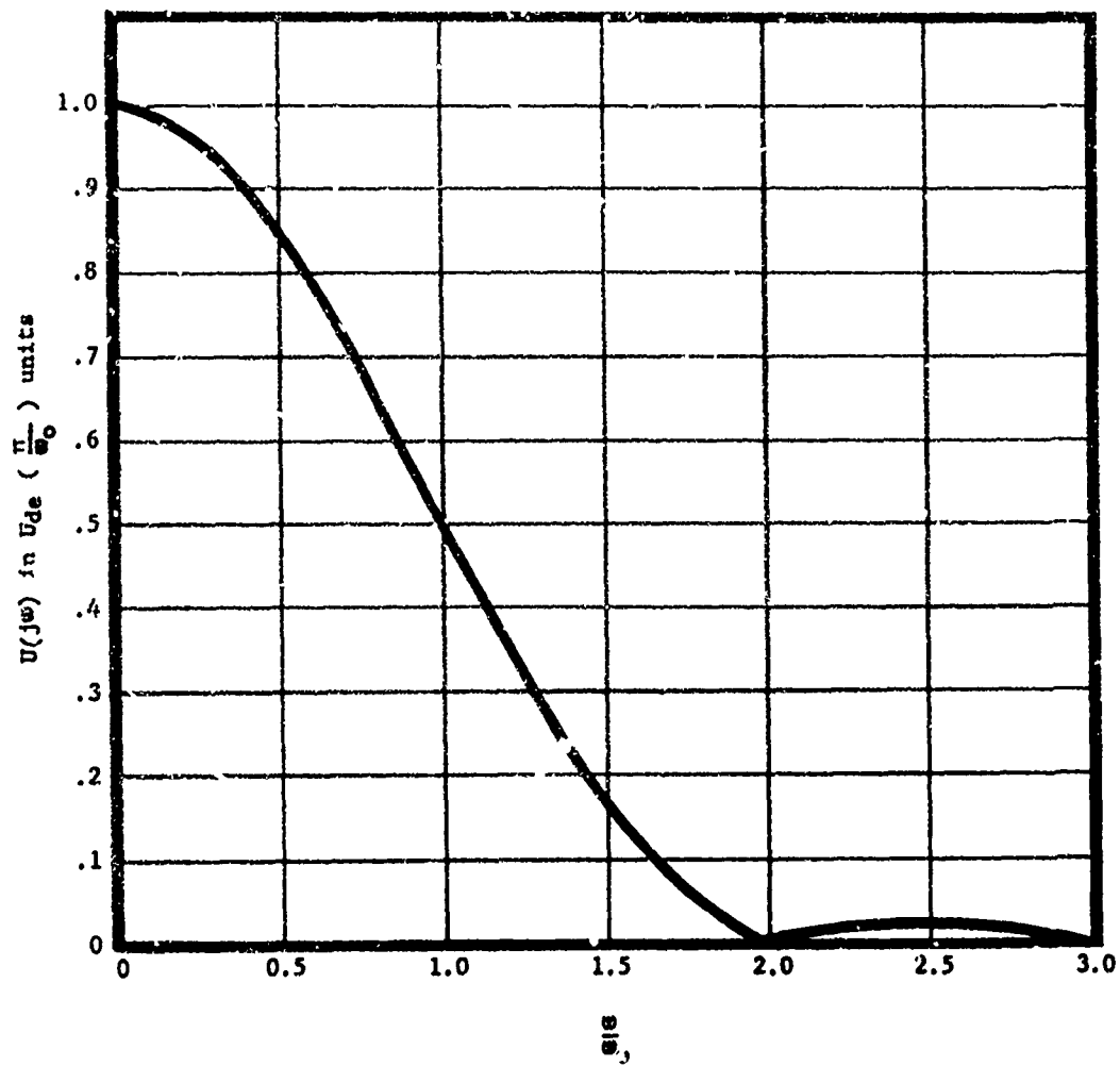
Figure 31. Frequency Content of 1-cos Impulse
