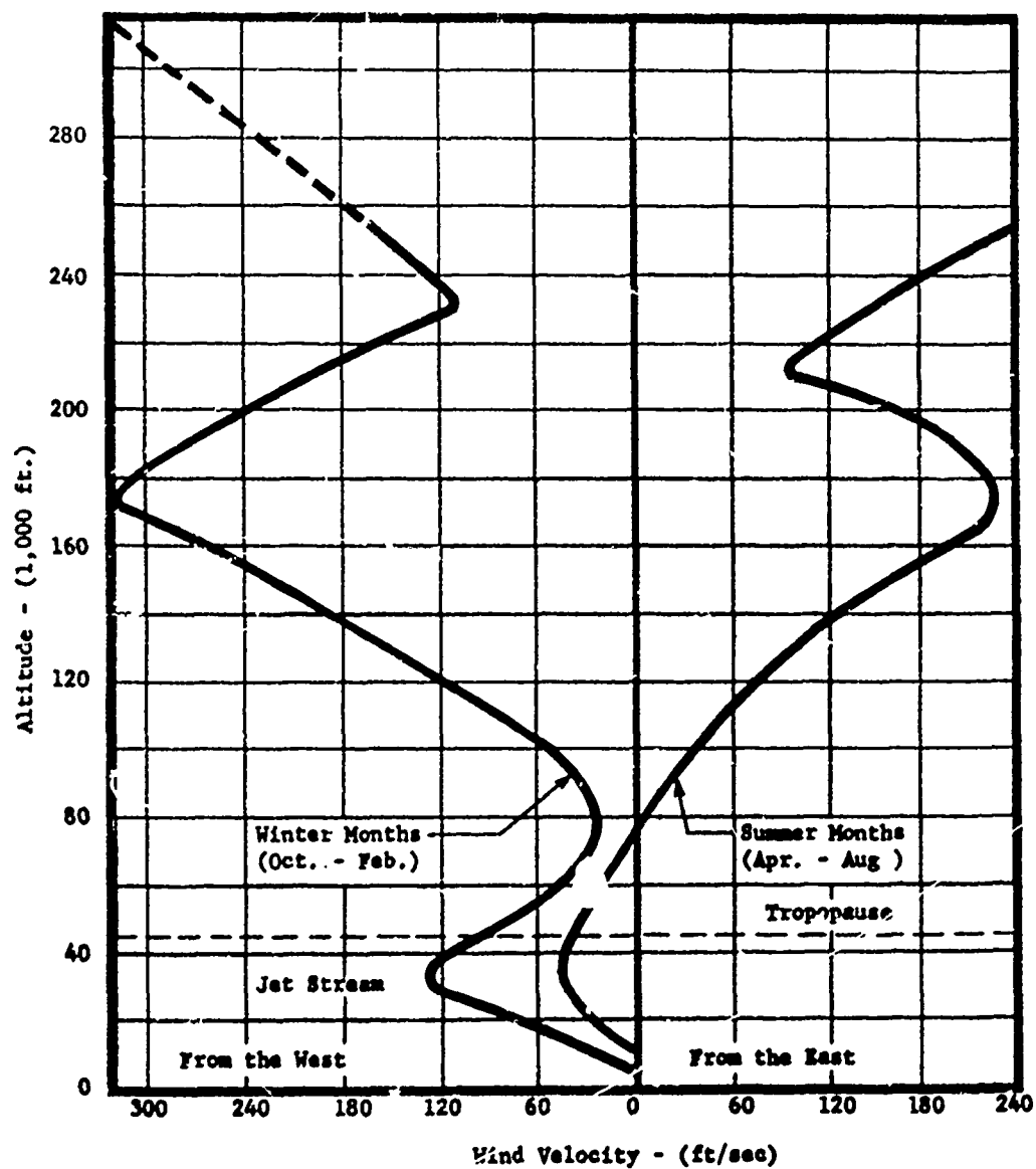
Figure 4. Average General Wind Profile
