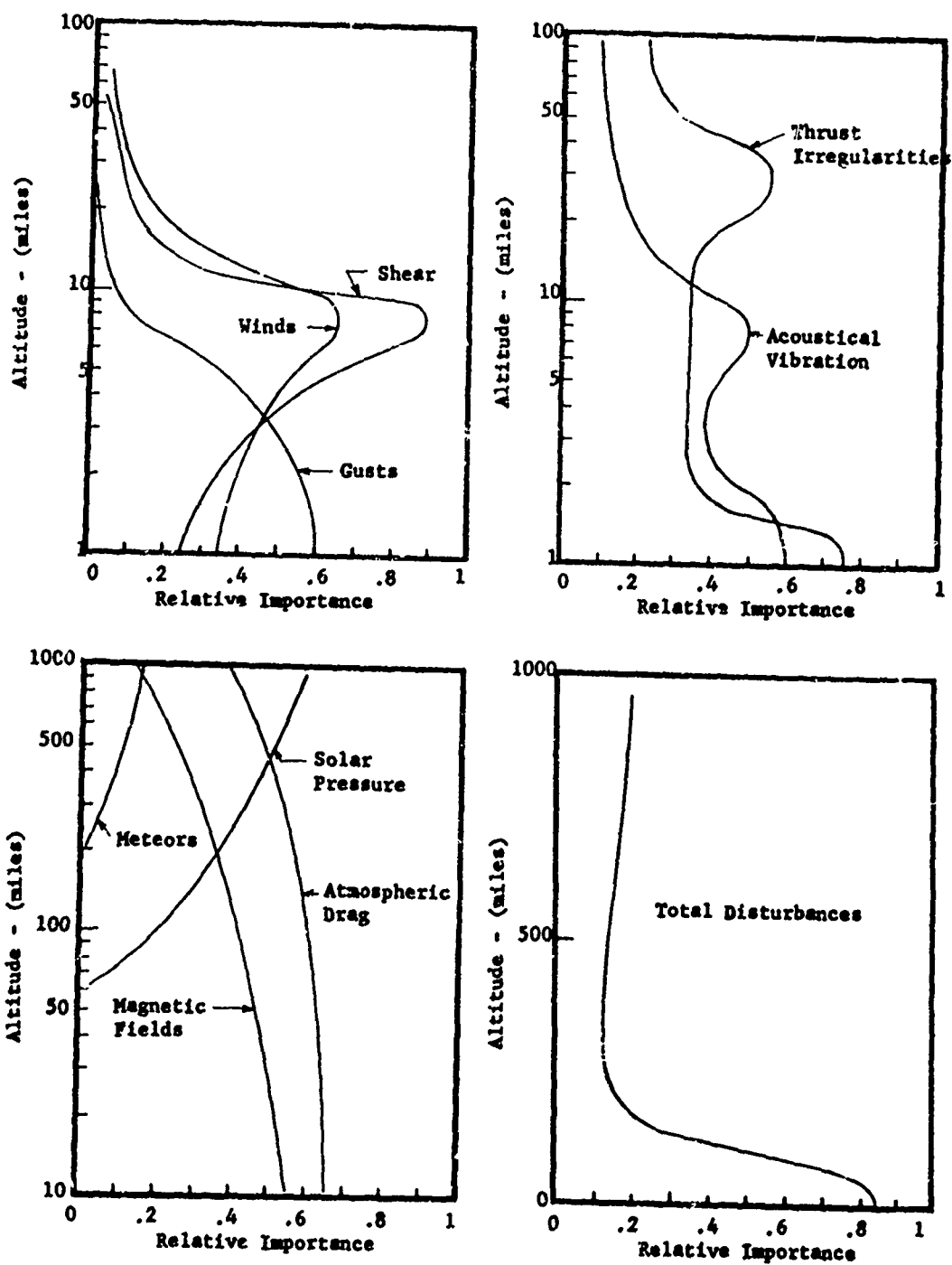
Figure 2. Relative Importance of Disturbances with Altitude.
