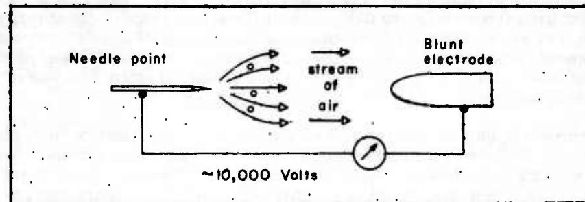
Figure 1. Corona wind from a charged point
