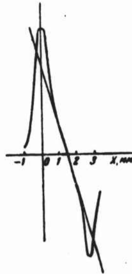
Fig. 2. Lateral photovoltaic effect related to light spot position on cell surface according to Taubkin and Frimer [1 1964 ]
