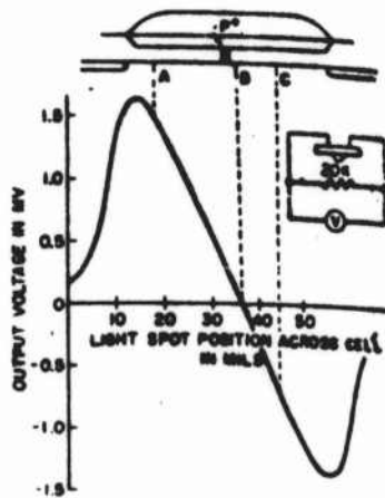
Fig. 1. Lateral photovoltaic effect in relation to light spot position on cell surface according to Wallmark [2 1968 ]
