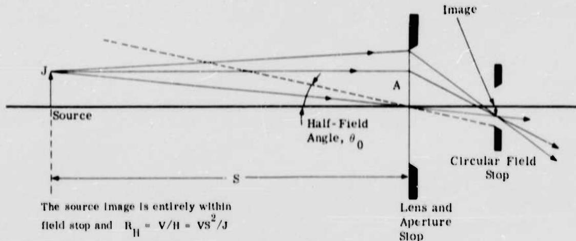
FIGURE 2. DISTANT SMALL-SOURCE CALIBRATION
