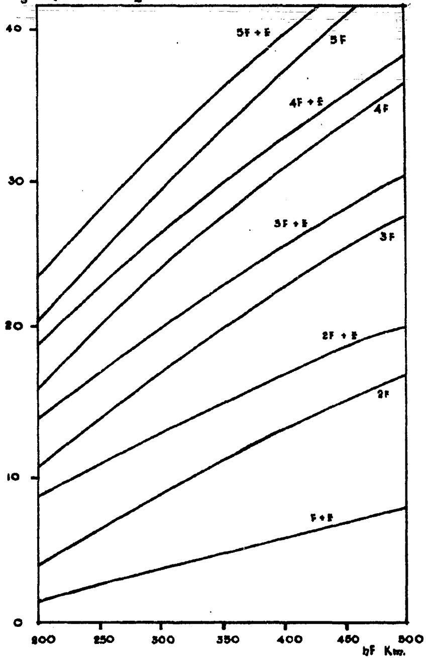
FIG.10 ANGLE OF ARRIVAL V. REFLECTION HEIGHT FOR FREIBURG-ACCRA (4460km)
