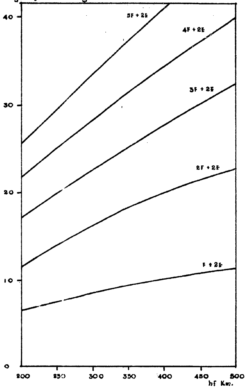
FIG. II ANGLE OF ARRIVAL V. REFLECTION HEIGHT FOR FREIBURG—ACCRA (4660 Km.)
