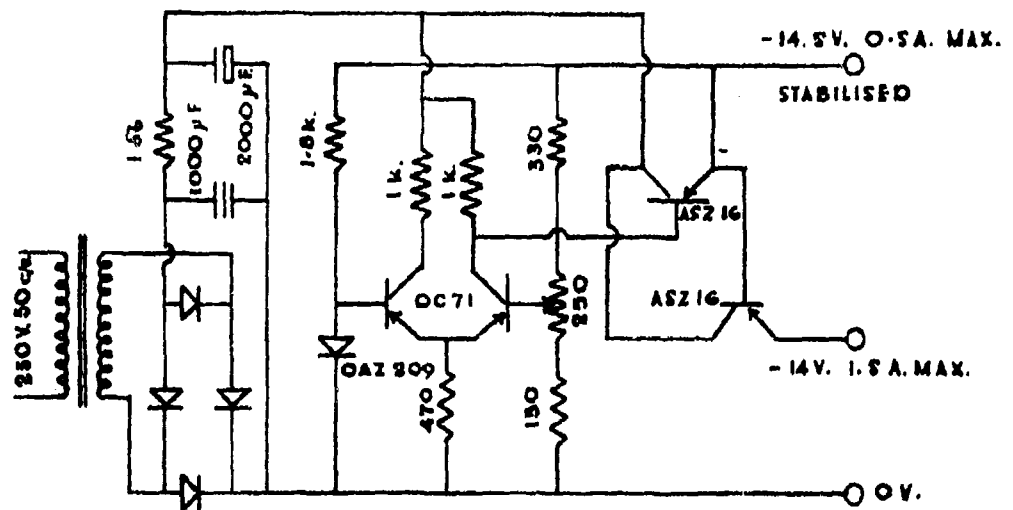
FIG. 6 POWER SUPPLY FOR TEMPERATURE - SENSITIVE AMPLIFIER.
