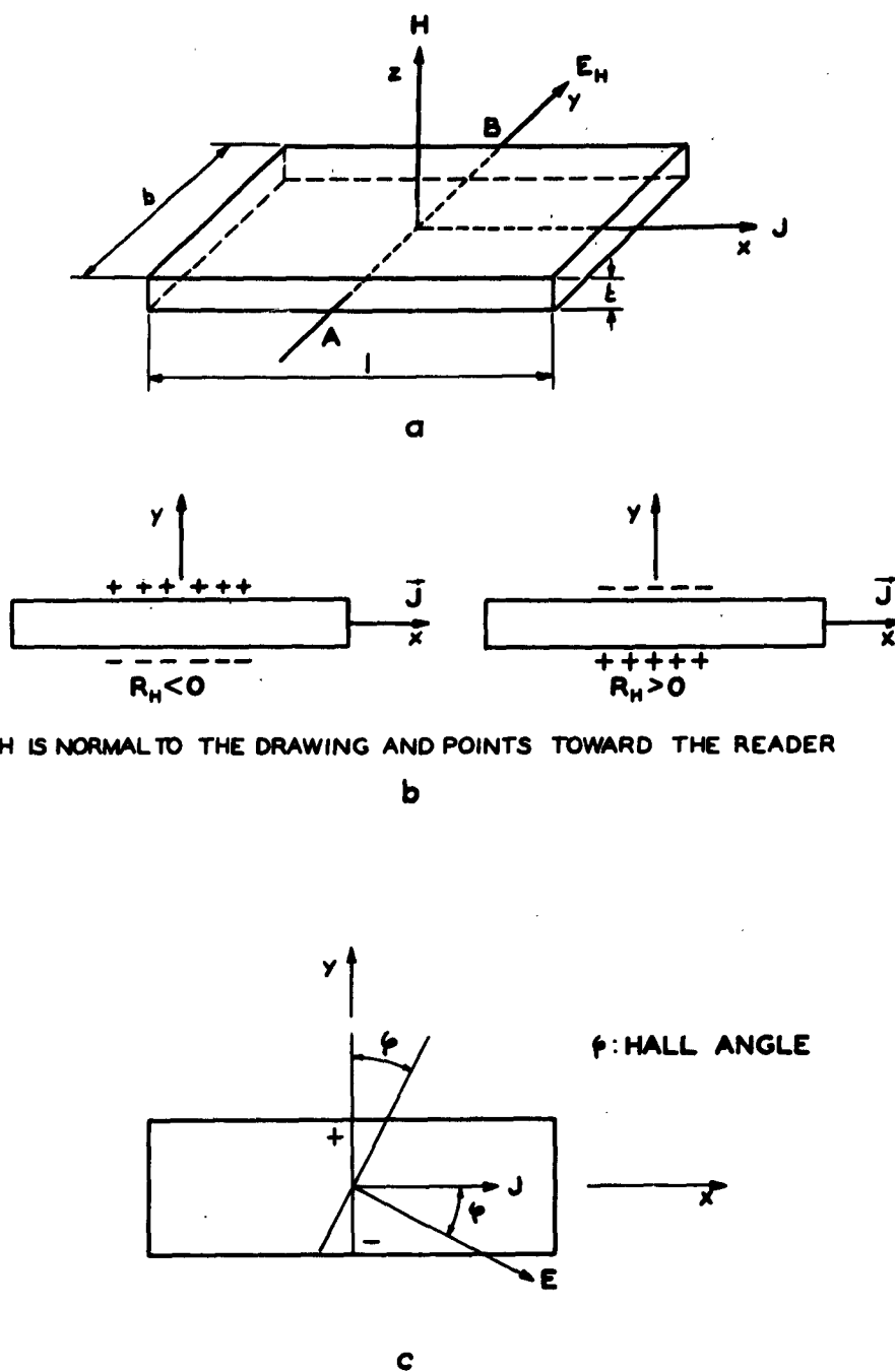
Fig. 3. a. Geometry of a Hall measurement specimen b. Sign of the Hall coefficient c. Hall angle
