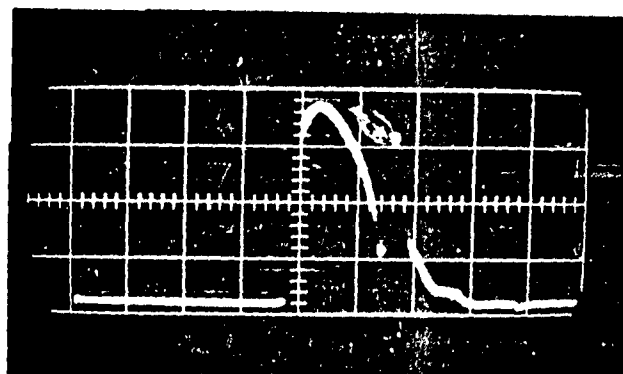
(b) Probes 3.15 cm from filter, receptor length 3.8 cm, S_1/S_1^* = 0.96 .
