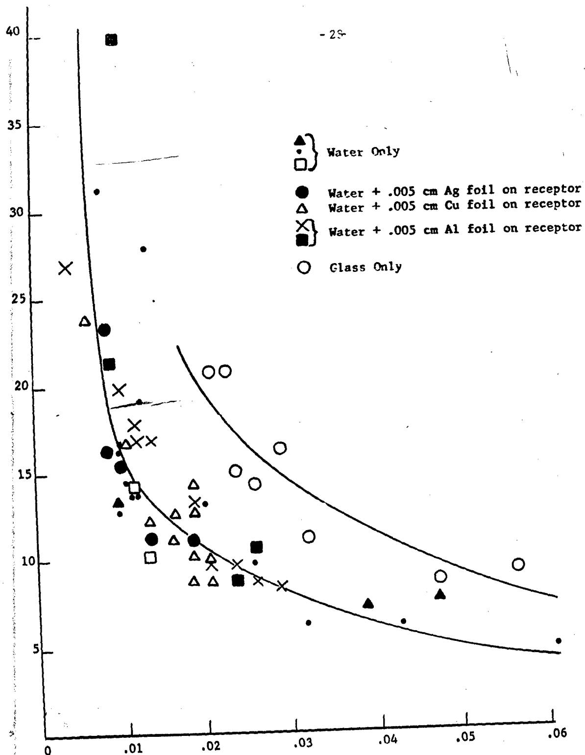
Fig. 15: Initial peak conductance vs time to detonation from parallel probes in 2" (d) x 8" (L) Composition B charges using water or glass barriers.
