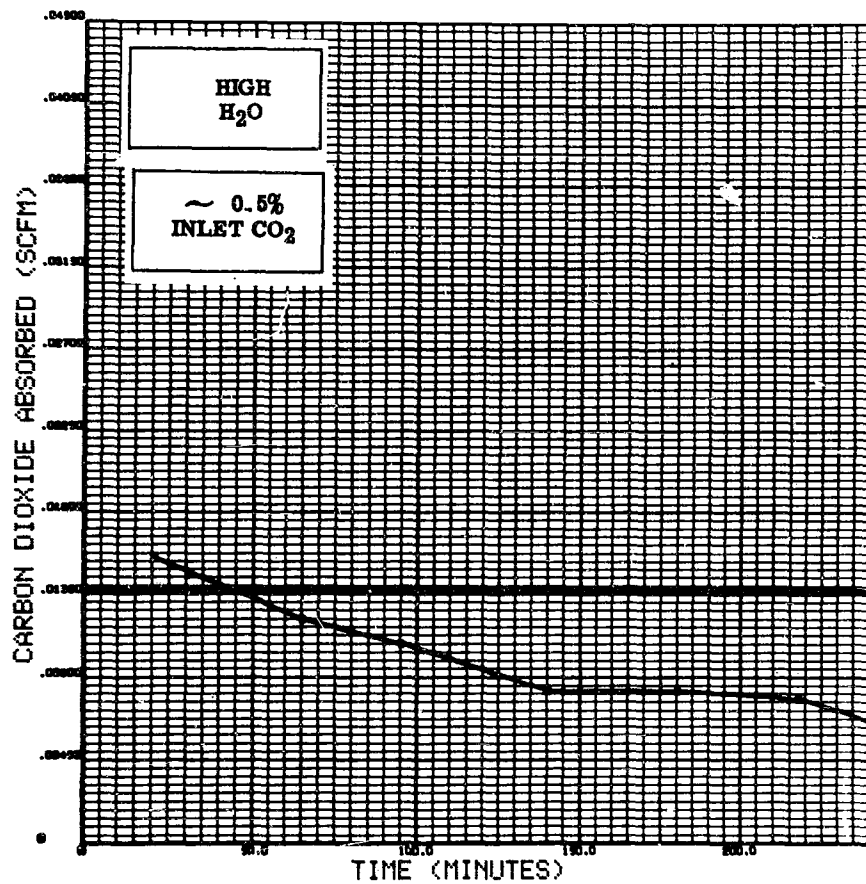
Figure 69 SC-4020 Curve, CO 2 , P-4, B
