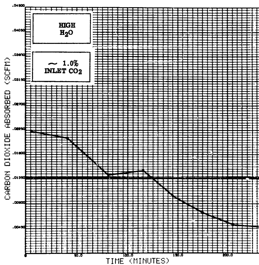
Figure 49 SC-4020 Curve, CO 2 , P-1, MSA
