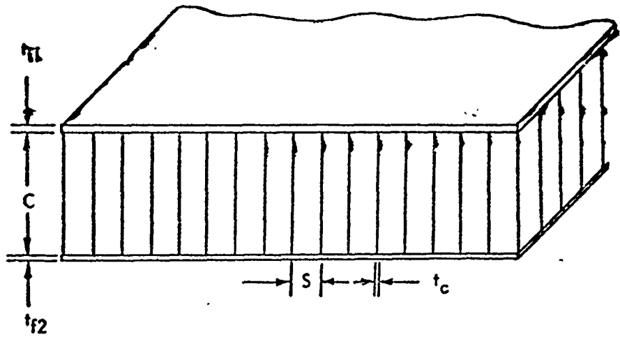
HONEYCOMB PANEL
