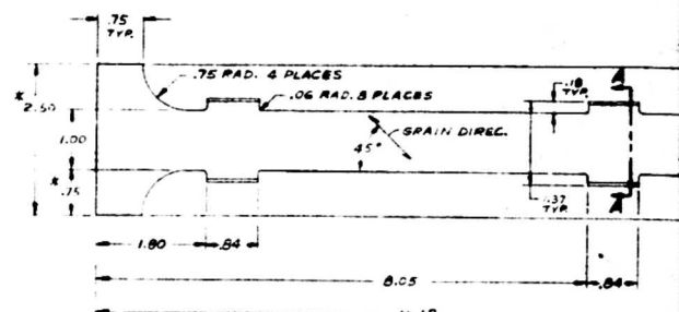
DETAIL -19 DOUBLER IDENTICAL TO -15 DBLR EXCEPT FOR THESE DIMS.
