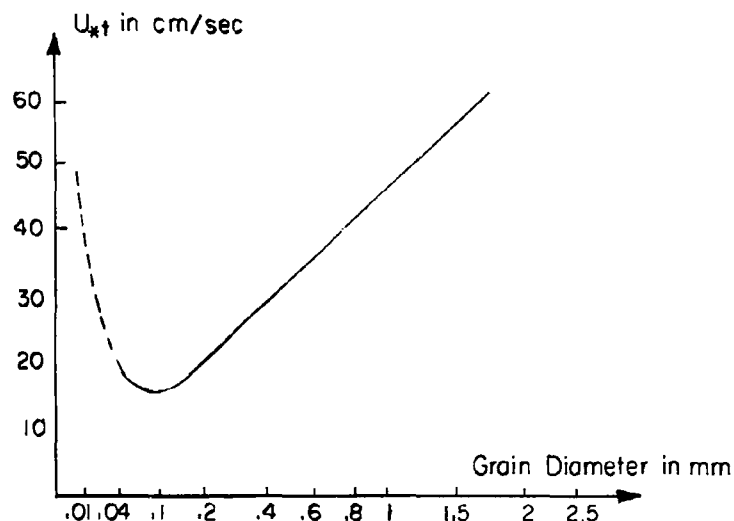
FIGURE 1- INITIATION OF SAND MOVEMENT
