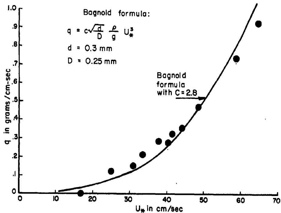
FIGURE 4 - COMPARISON BETWEEN EXPERIMENTAL RESULTS H8896 A AND BAGNOLD FORMULA
