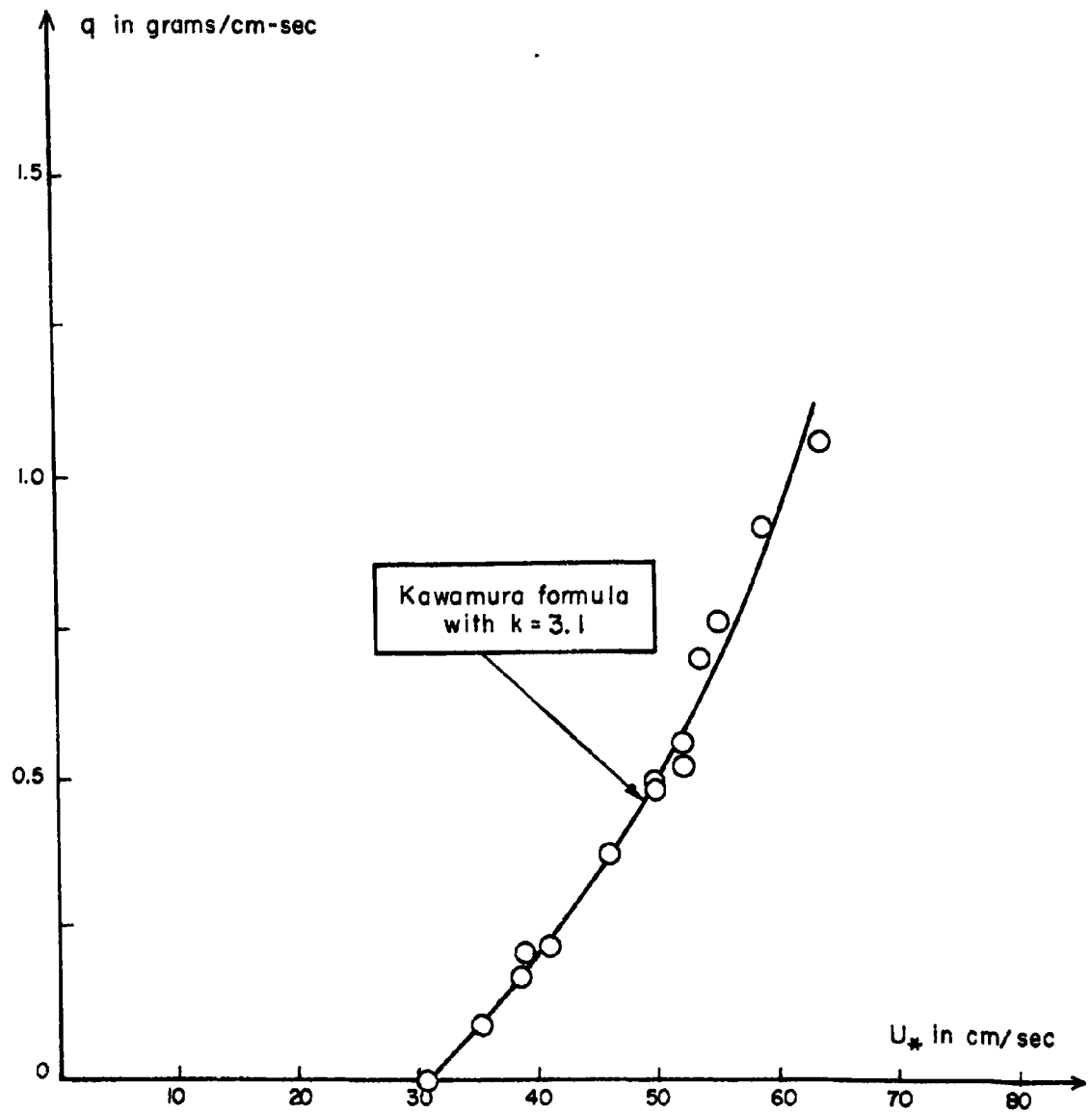
FIGURE 18- COMPARISON BETWEEN EXPERIMENTAL RESULTS AND THE KAWAMURA FORMULA
