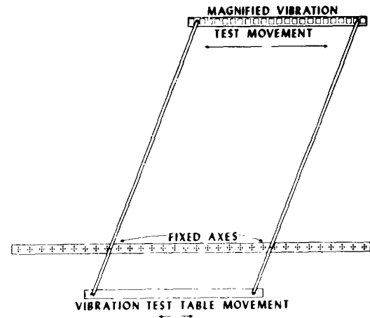
Figure 2. Amplitude Magnifier.
