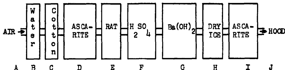
Figure 2. Respiration Train
