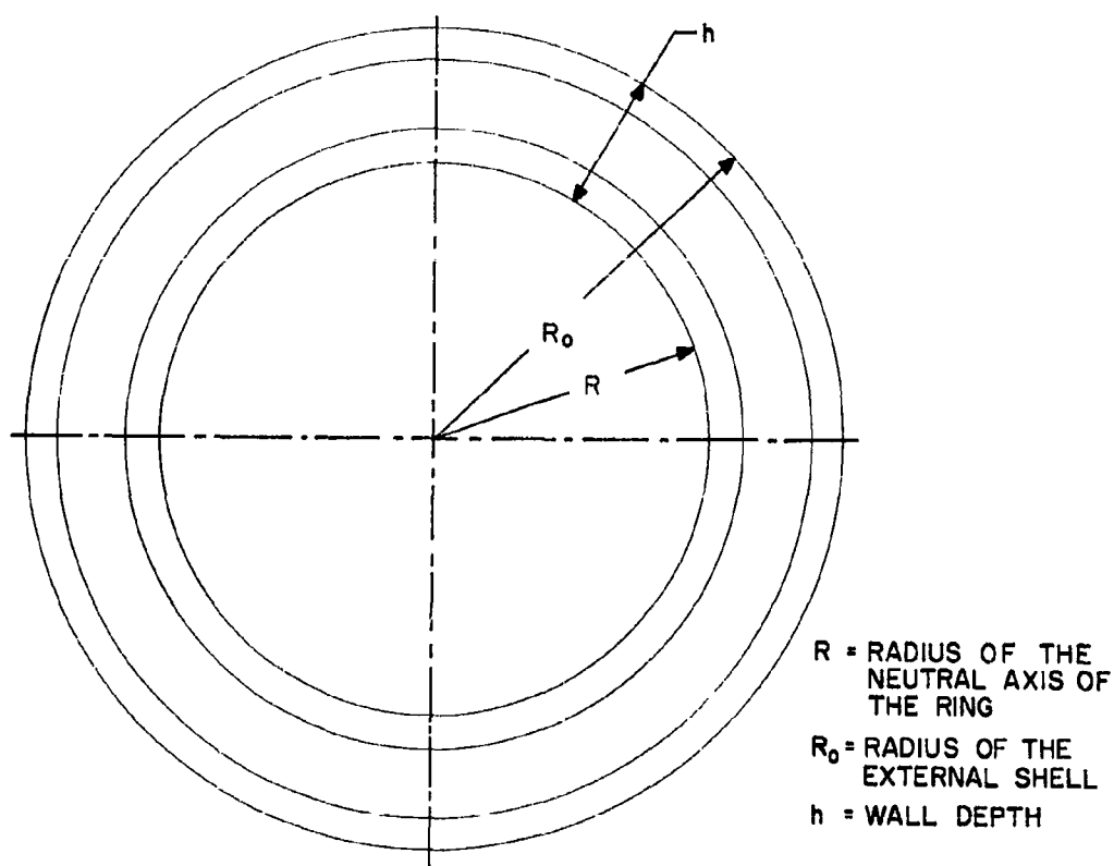
Fig. 2 - Structure of Cellular Sandwich Shell
