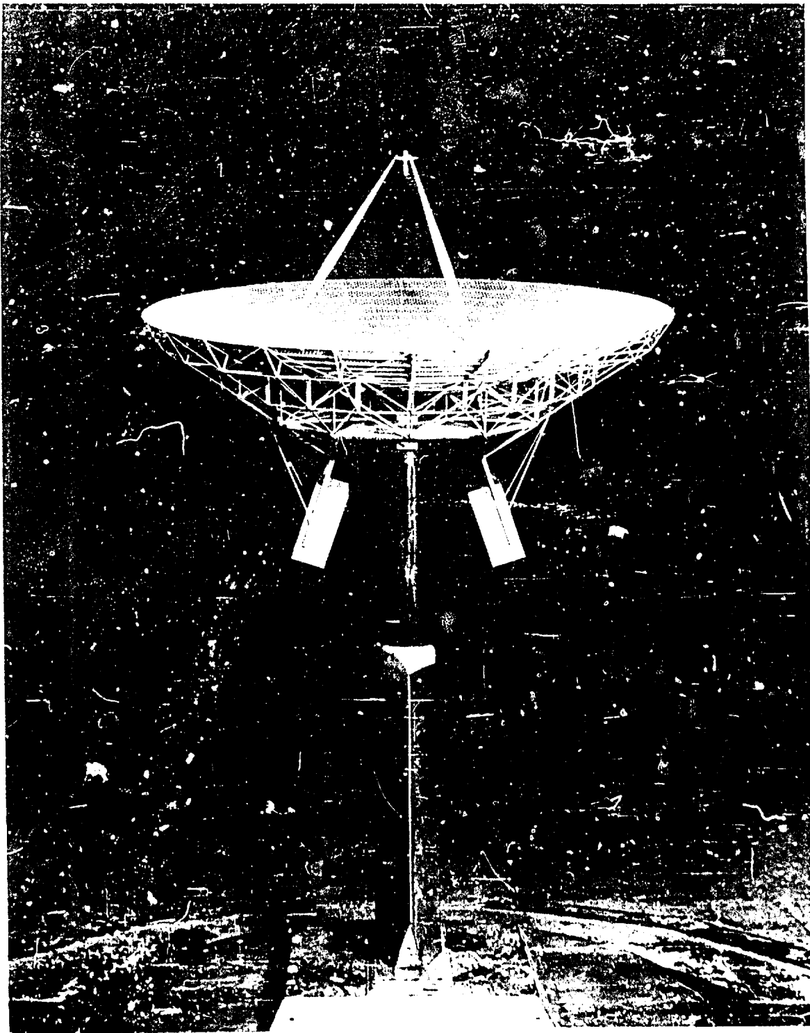
Fig. 3 Mesh Reflector MRF \psi = 180 , \theta = 80 View Looking Upstream.
