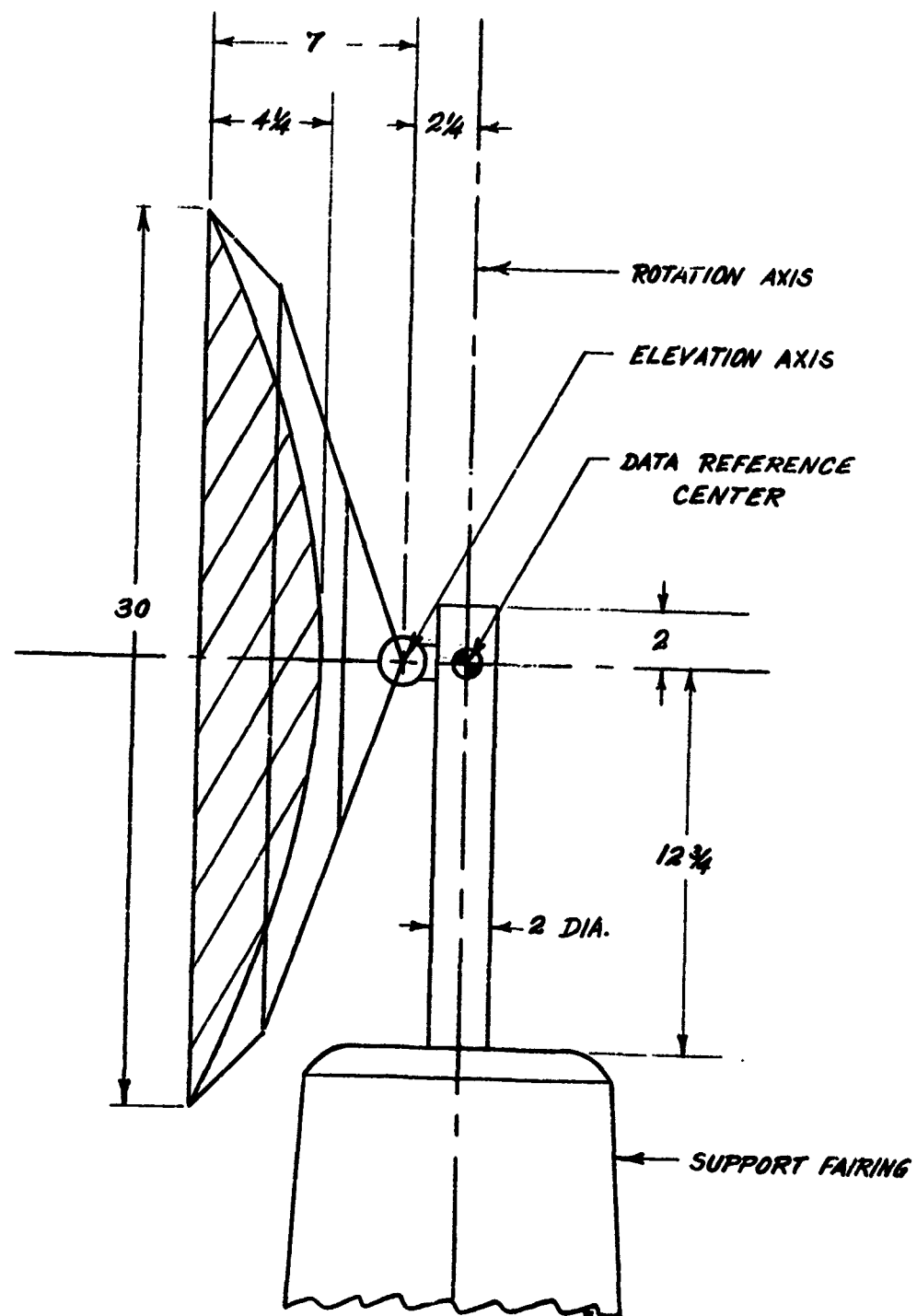
Fig. 4 NOTE: ALL DIMENSIONS IN INCHES SCALE . 1/5
