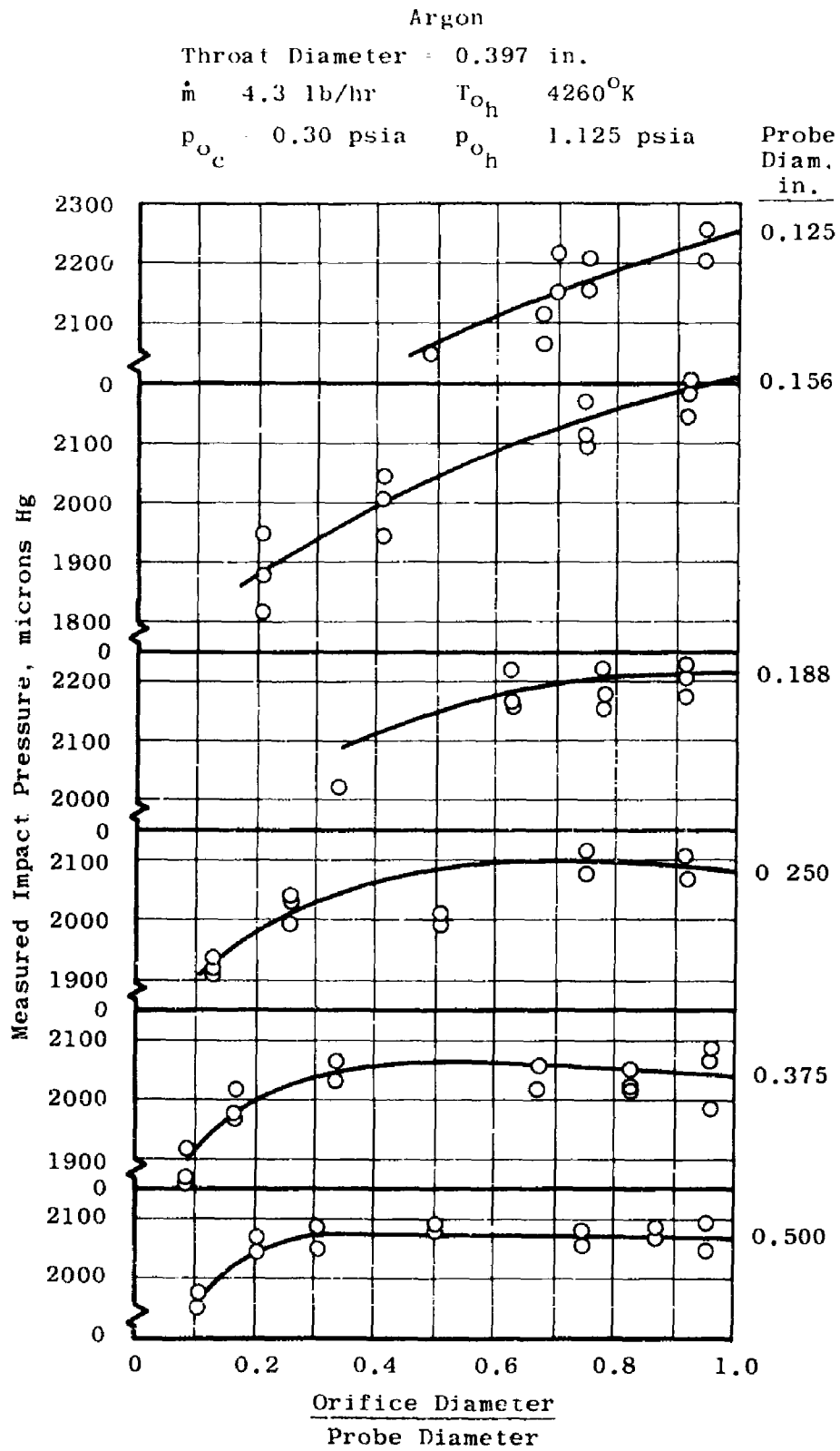
Fig. 2a Variation of Measured Impact Pressure with Orifice-to-Probe Diameter Ratio
