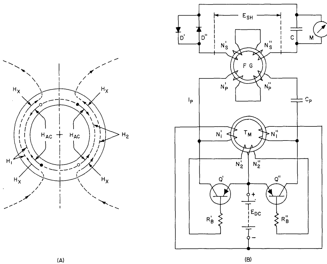
Fig. 14 Ring-core flux-gate magnetometer. (A) Fundamental principle. (B) ac excitation with switching-transistor magnetic-coupled multi-vibrator.
