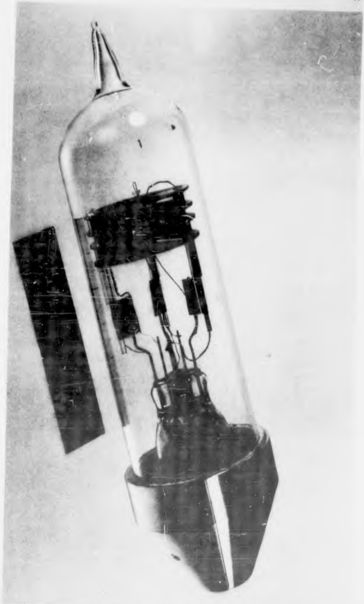
Figure 13 - Completed G12x-R tube with special base.
