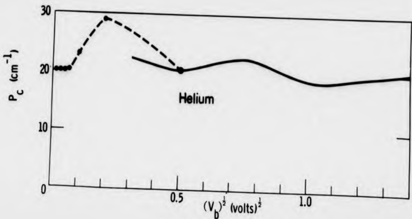
Figure 3 - Collision probability in helium.
