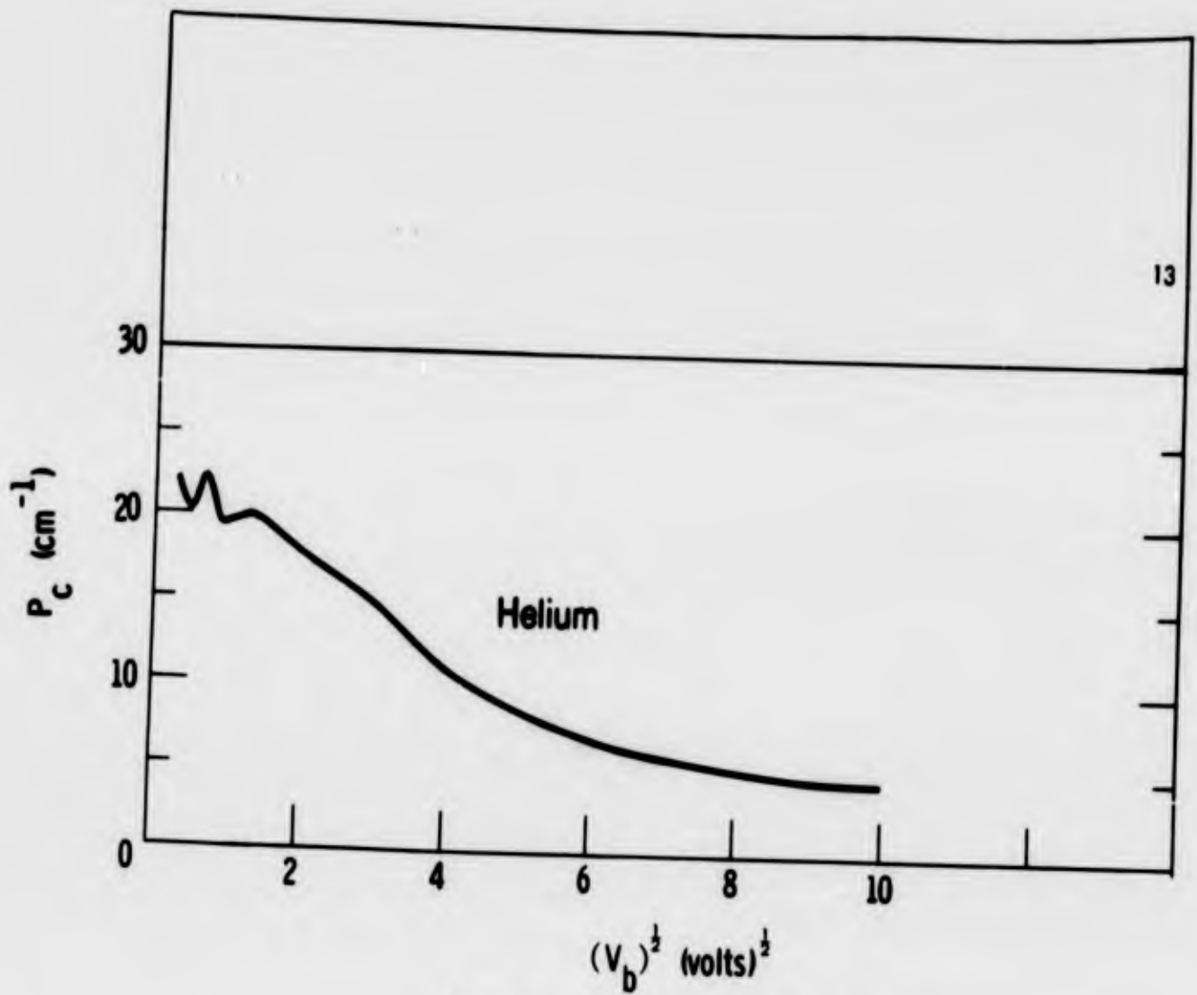
Figure 2 - Collision probability in helium.
