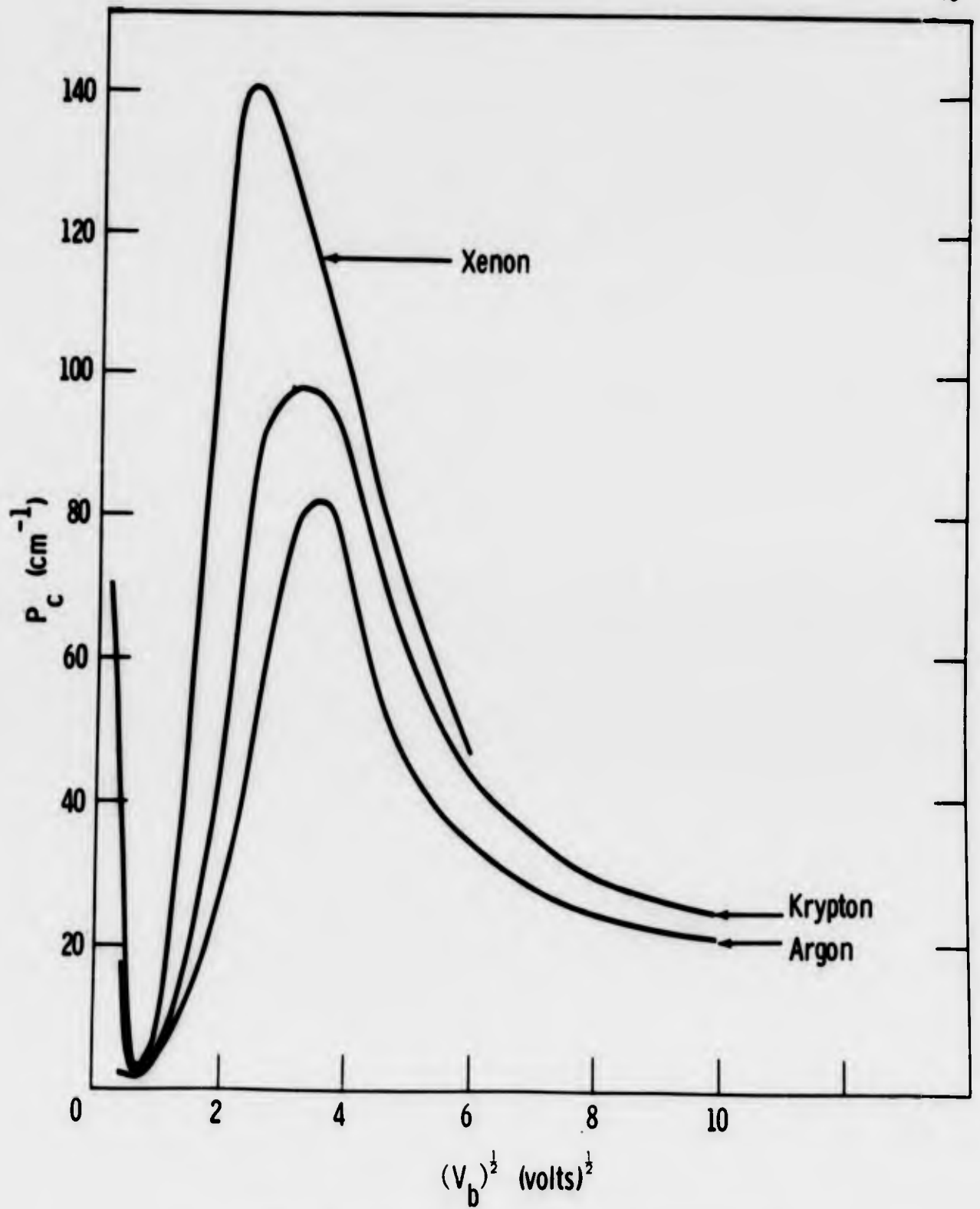
Figure 10 - Collision probability in xenon, krypton and argon.
