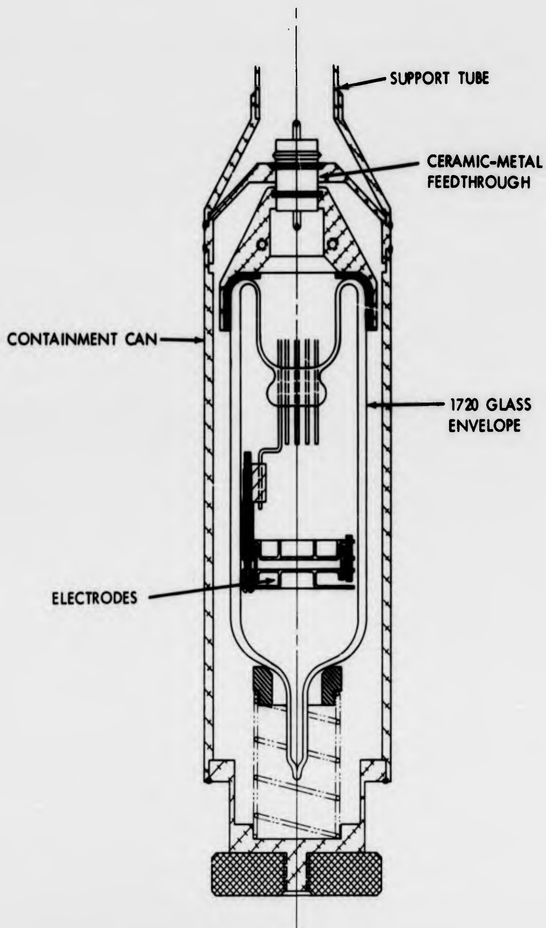
Figure 11 - Details of inpile ion chamber G12x-R.
