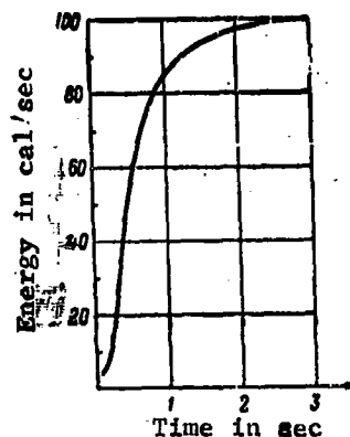
Fig. 48. Proportion of luminous energy de-excited by different moments of time during explosion of a bomb with TNT equivalent of 20,000 tons.
