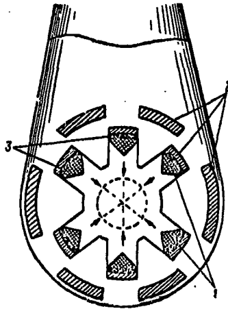
Fig. 7. Simplified diagram of atomic bomb: 1) uranium or plutonium; 2) conventional explosive; 3) neutron reflector.
