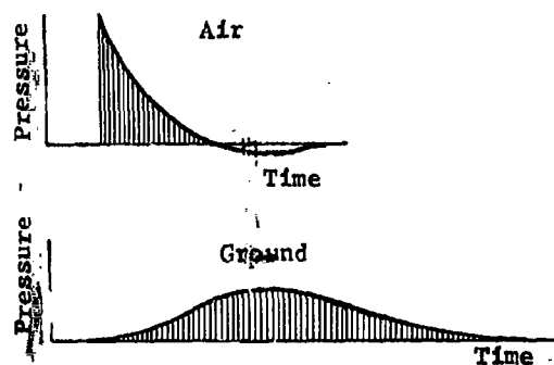
Fig. 41. Variation in pressure in air and in ground during explosion.
