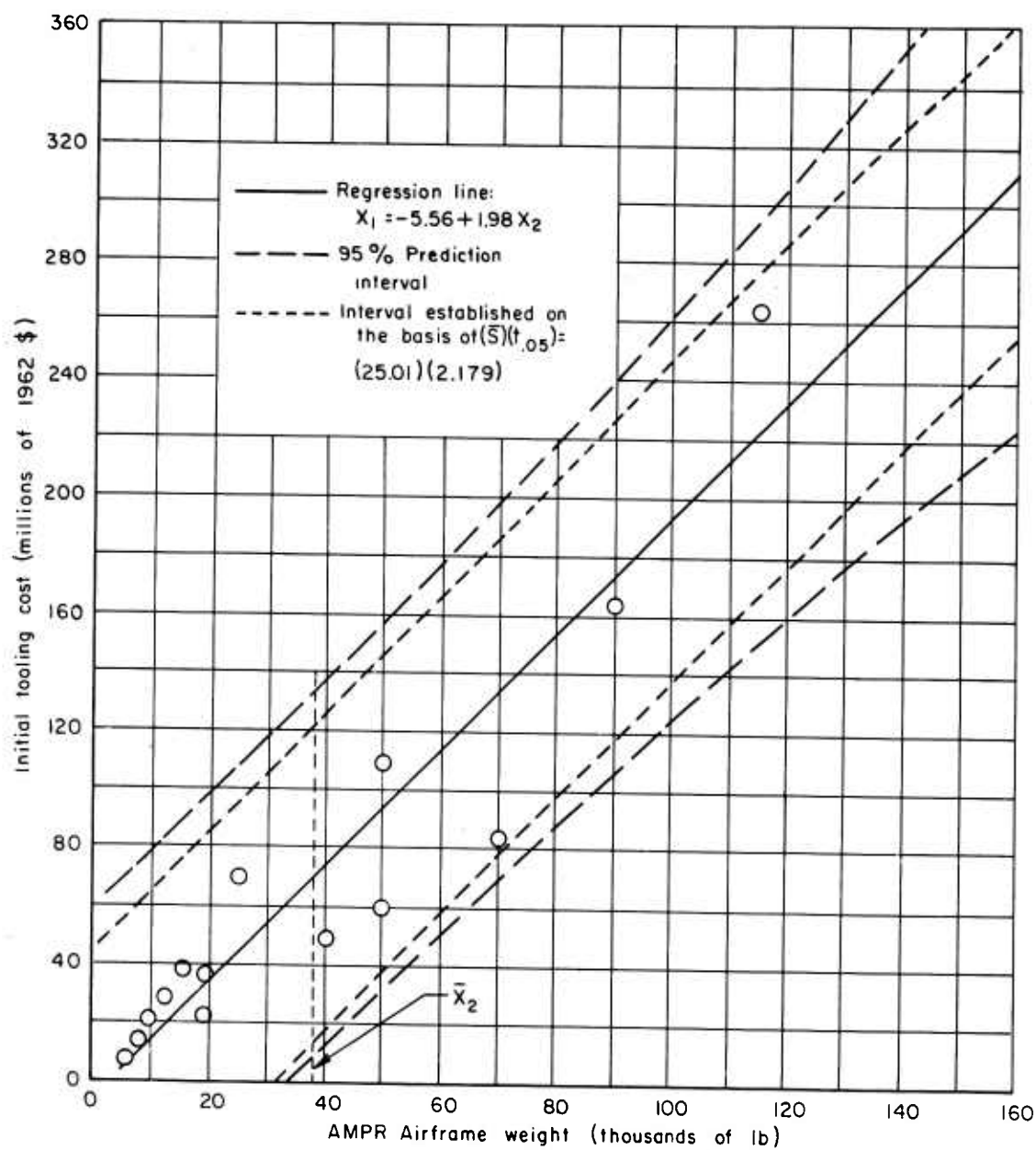
Fig. 6.—Initial tooling cost versus airframe weight
