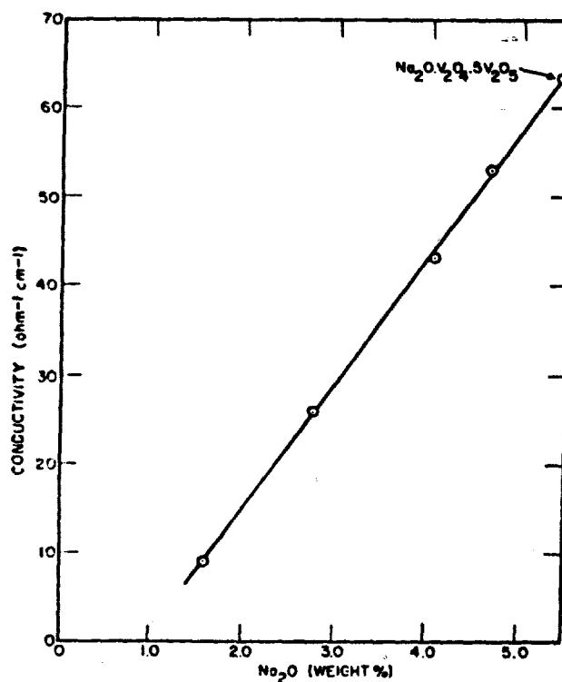
Fig. 4 - Electrical conductivity as a function of sodium content in the system \text{Na}_2\text{O}-\text{V}_2\text{O}_5(3)
