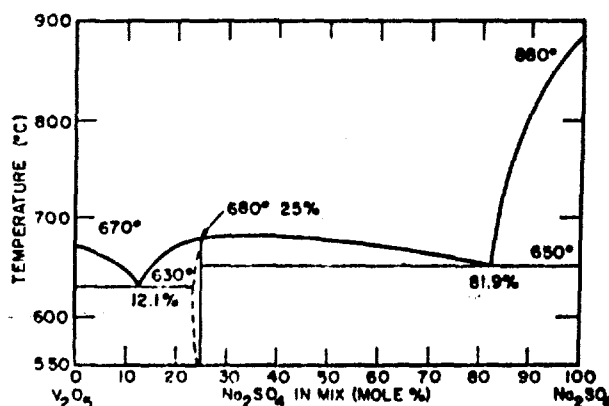
Fig. 3 - Phase diagram for the system \text{Na}_2\text{SO}_4 - \text{V}_2\text{O}_5 (Obtained from heating curves. Systems not at equilibrium.) (1)
