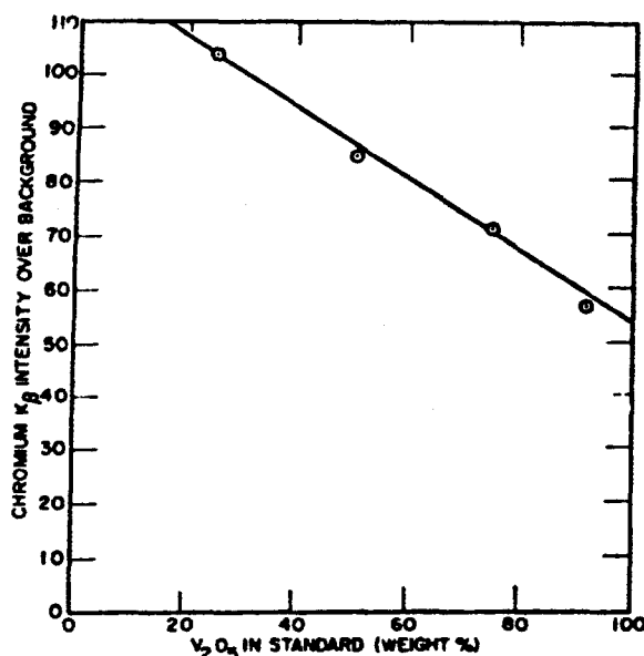
Fig. 6 - Typical calibration curve for estimating vanadium content of oil ash by absorption of chromium K β radiation
