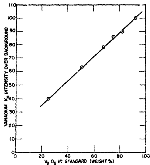
Fig. 7 - Typical calibration curve for estimating vanadium content of an oil ash by direct measurement of secondary vanadium radiation
