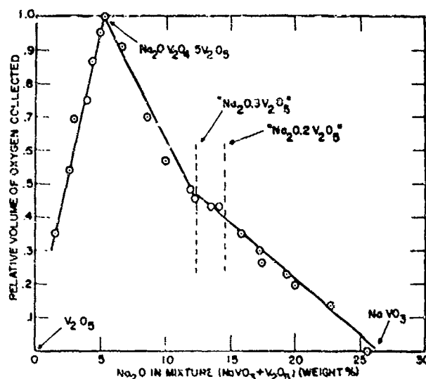
Fig. 5 - Oxygen evolution as a function of sodium content of melts containing sodium and vanadium oxides (3)
