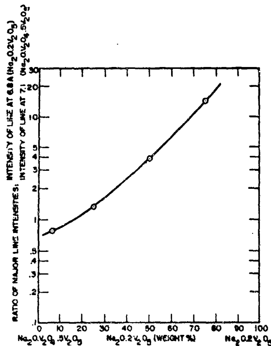
Fig. 8 - Calibration curve for the estimation of two oxides of sodium and vanadium by an x-ray powder diffraction method
