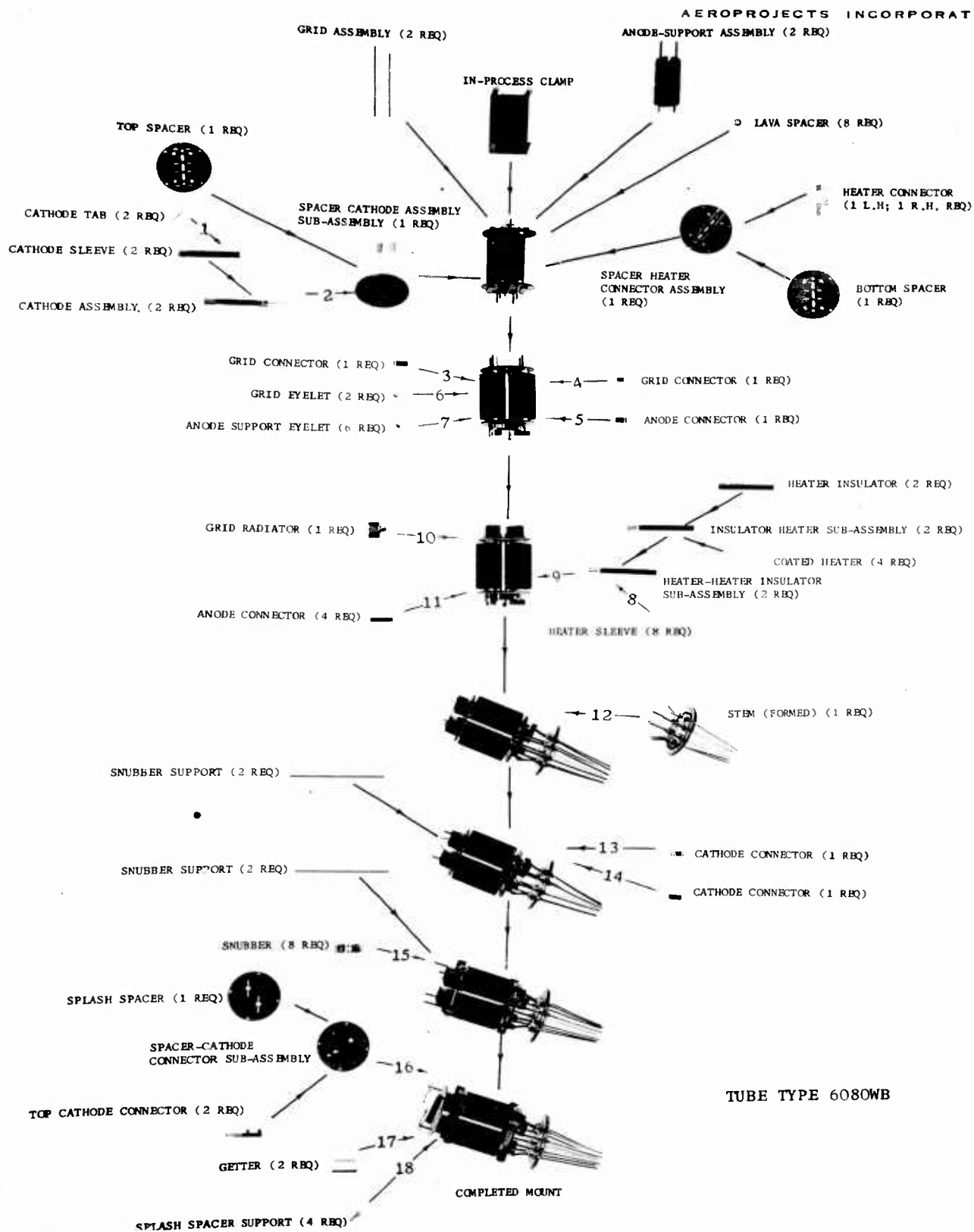
Figure 14 TUBE ASSEMBLY SEQUENCE
