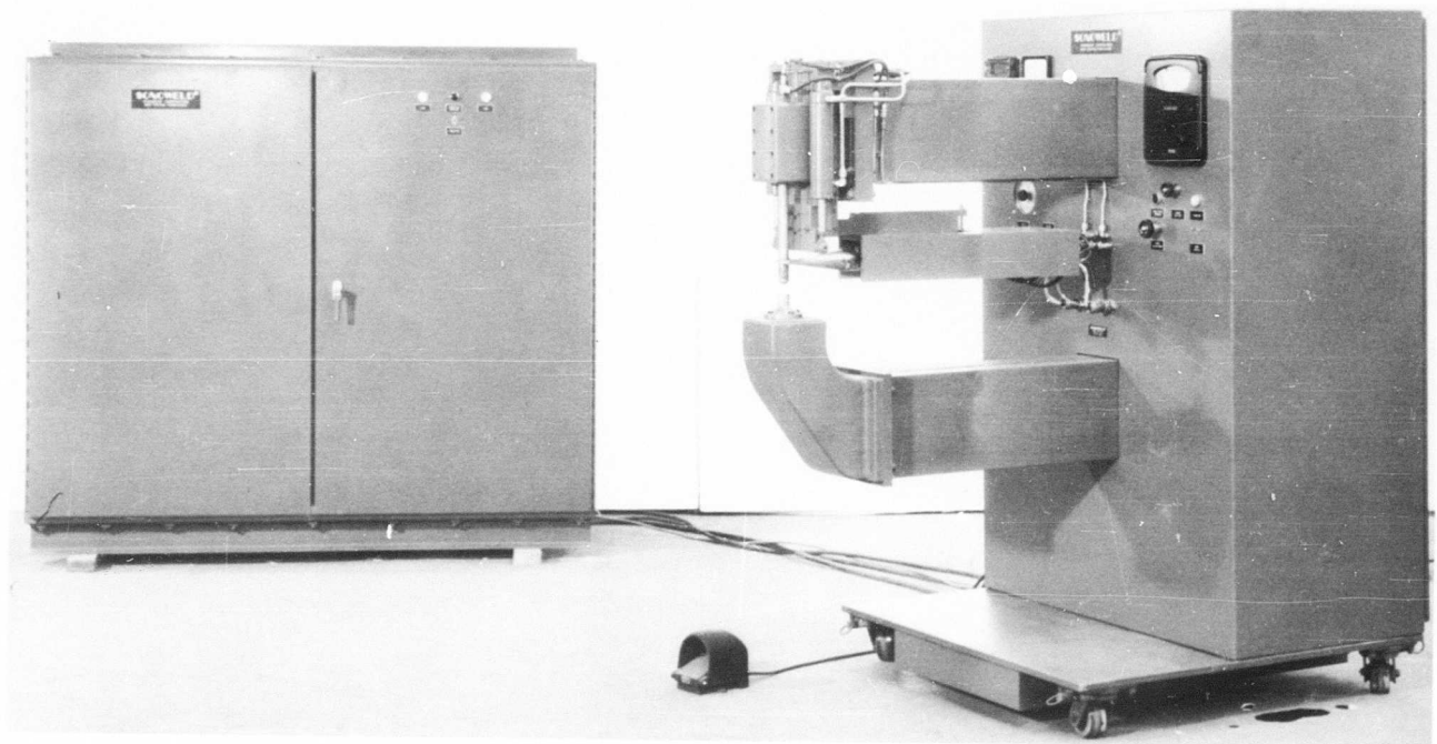
4-kw welder
