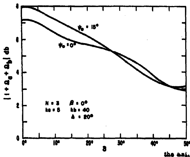
Fig. 11 The amplitude of 1 + \Omega_g + \Omega_b as a function of \theta/\delta for nonconducting ground illustrating the effect of finite \psi_0 for kb = 40
