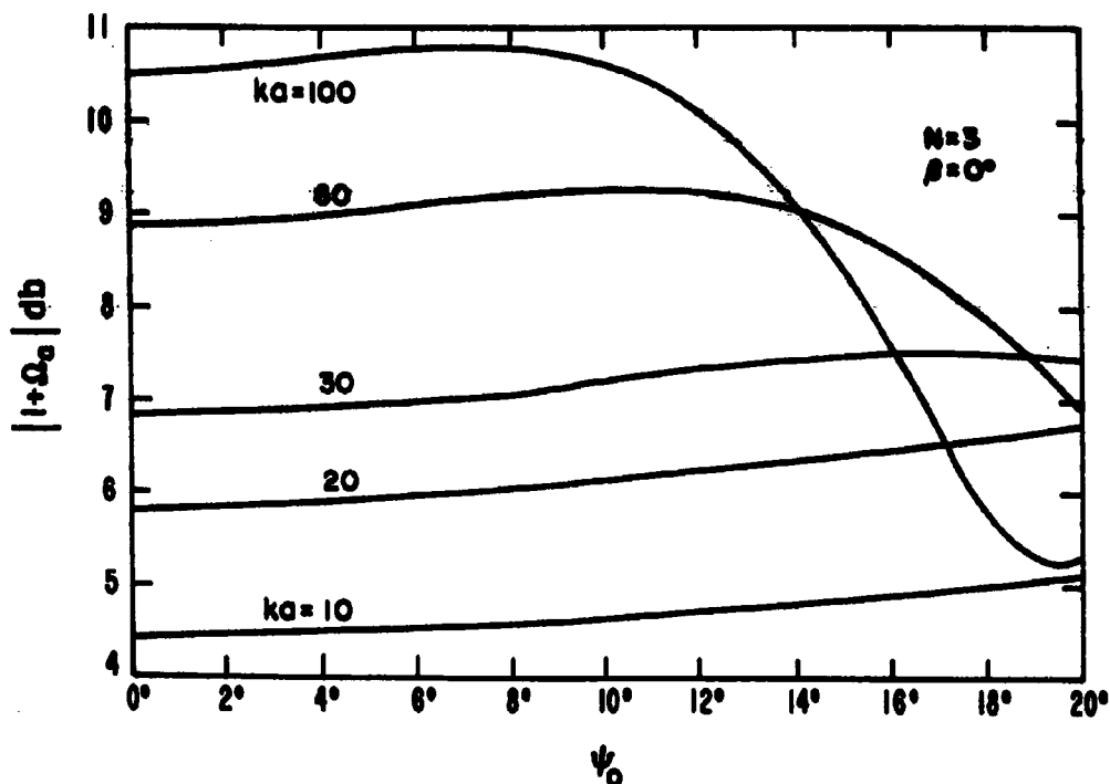
Fig. 2a The amplitude of 1 + Q_g as a function of \psi_0 with parameter ka for nonconducting ground illustrating the effect of the circular screen of radius a . [The ordinate can be regarded as the modification of the effective height of the monopole resulting from the presence of the ground screen.]
