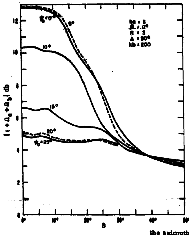
Fig. 12 The amplitude of 1 + \Omega_g + \Omega_b as a function of \theta/\delta for nonconducting ground illustrating the effect of finite \psi_0 for kb = 200
