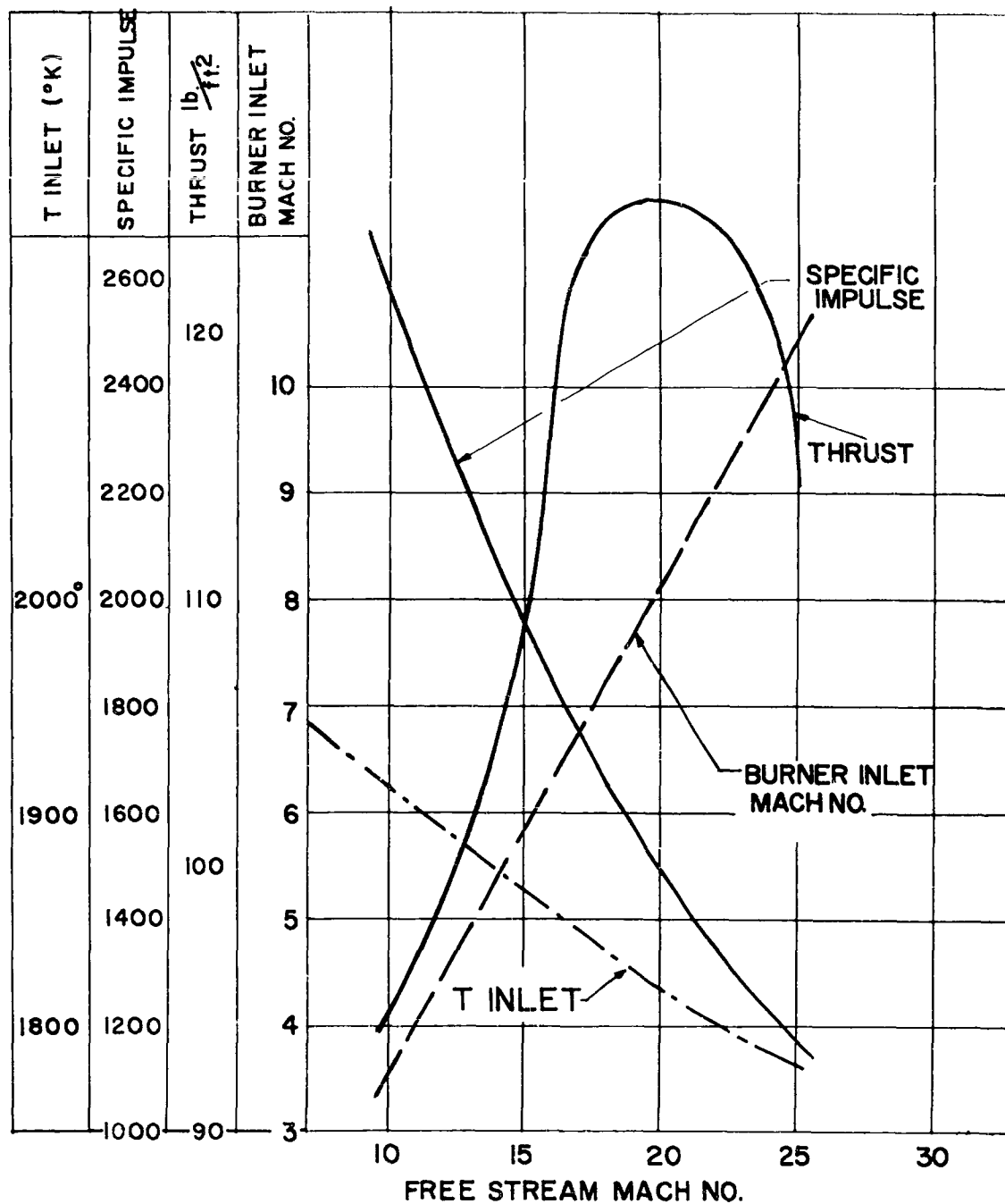
FIG. 1-2. Ramjet, Inlet Static Temperatures, Thrust, and Specific Impulse, for Various Free Stream Mach Numbers (Hydrogen Fuel), Altitude 150,000 ft.
