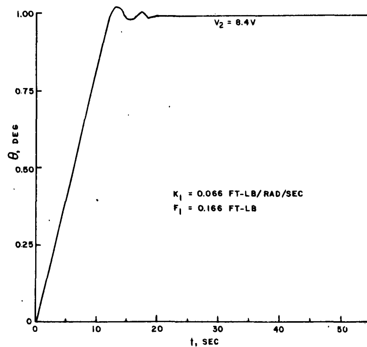
FIG. 15. Simulated System Response, Set No. 4.
