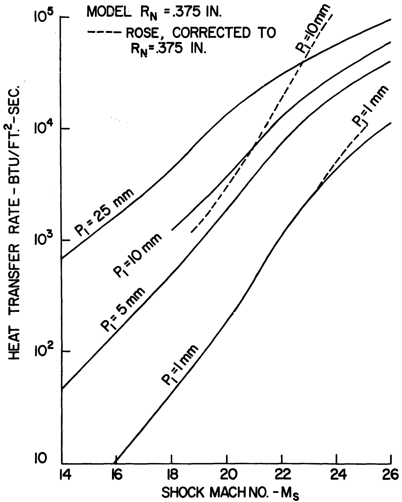
FIGURE 16 EQUILIBRIUM RADIATIVE HEAT TRANSFER AT THE STAGNATION POINT OF THE MODEL
