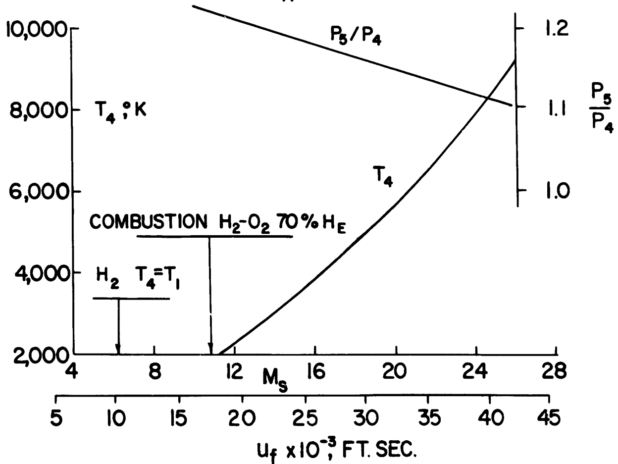
FIGURE 3 PERFORMANCE OF REFLECTED SHOCK TUNNEL TAILORED INTERFACE OPERATION
