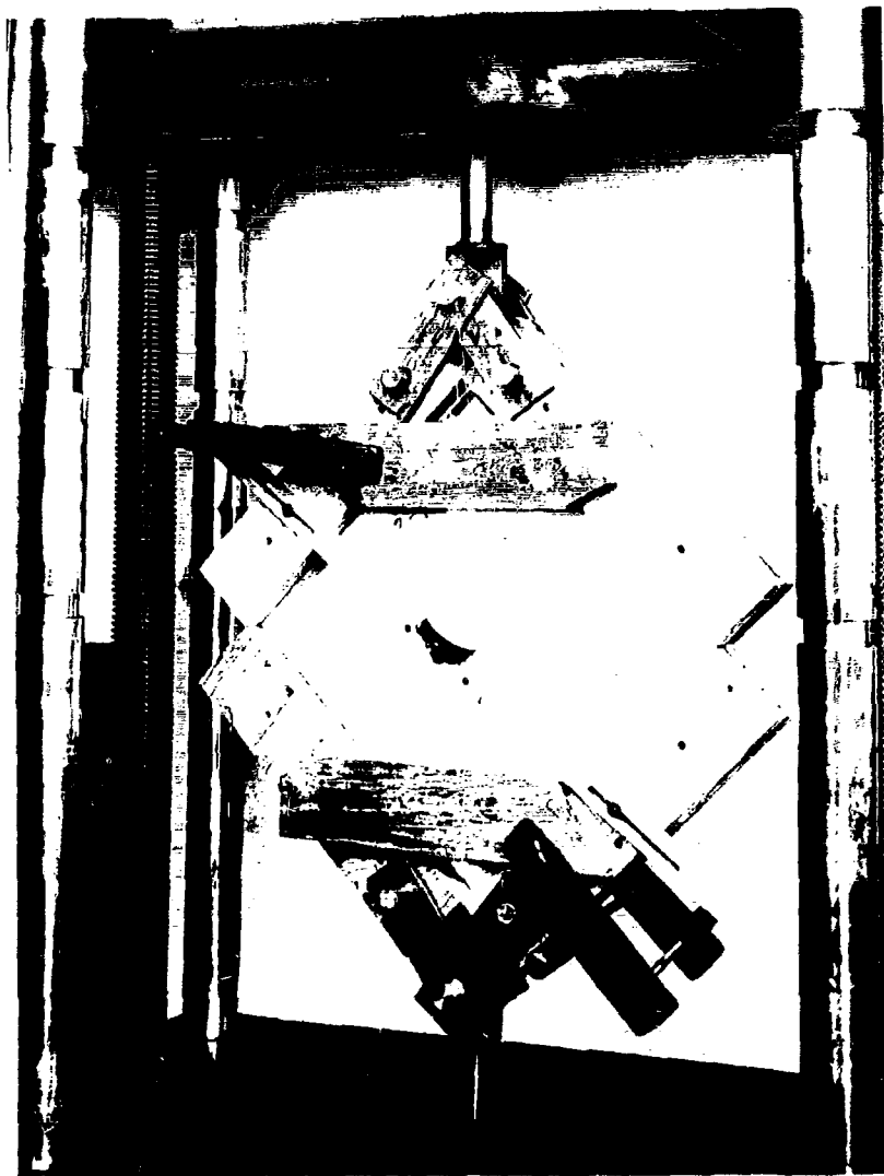
Figure 10. --Arrangement of apparatus for testing a square, flat panel of sandwich construction in shear.
