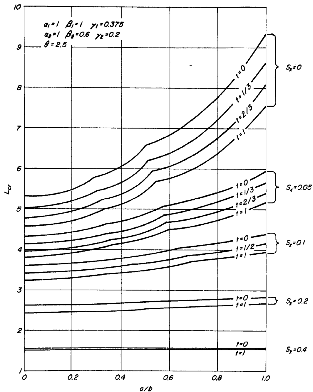
Figure 5. --Buckling coefficient, L_{cr} , for simply supported sandwich panels with orthotropic core in edgewise shear.
